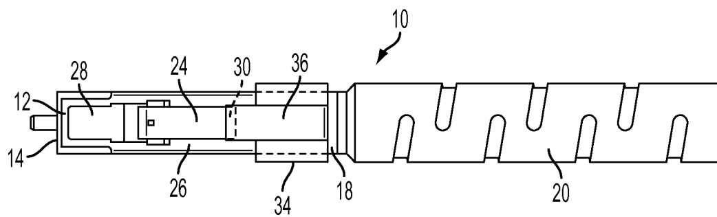
FIG. 2 CONVENTIONAL ART
