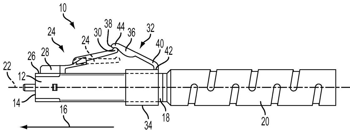
FIG. 1 CONVENTIONAL ART
