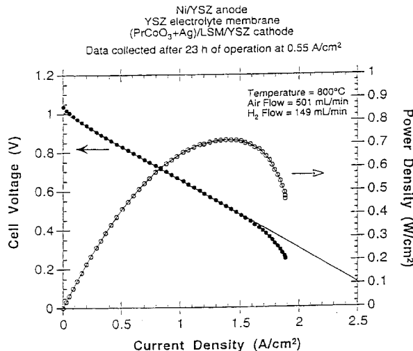
Fuel Cell of Example 1
