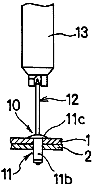
FIG. 95(b) (Prior Art)
