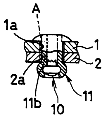
FIG. 94(f) (Prior Art)
