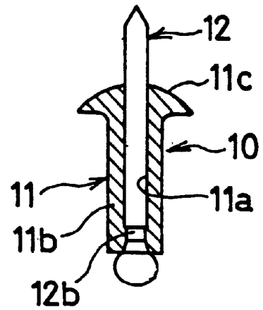
FIG. 94(c) (Prior Art)
