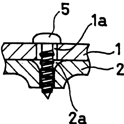
FIG. 92(b) (Prior Art)
