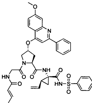
I-47
