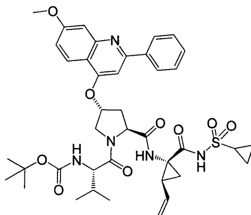
I-R
