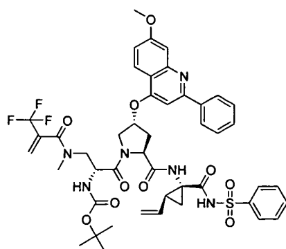
I-53
