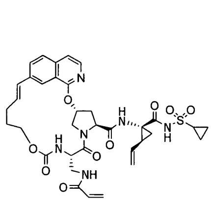
I-77
