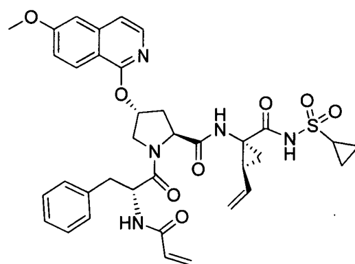
I-106
