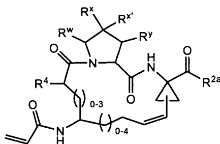
I-c-2
