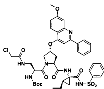
I-7
