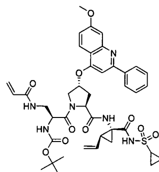
I-35
