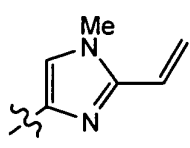
ggg
