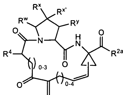
I-c-4
