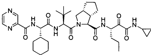
VX-950
