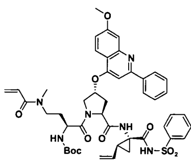
I-12
