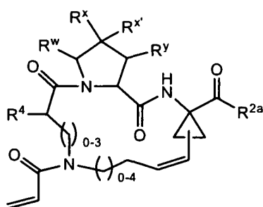
I-c-1
