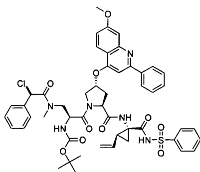
I-33
