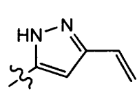
ddd
