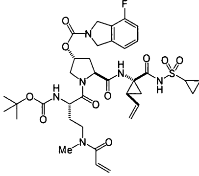
I-17
