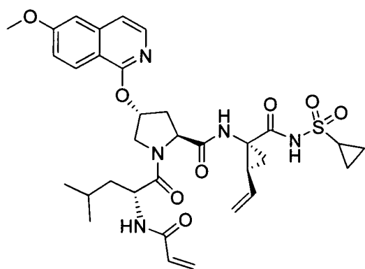
I-105
