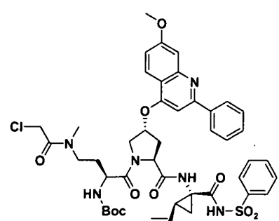
I-9
