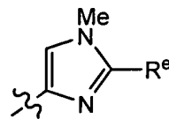
rr
