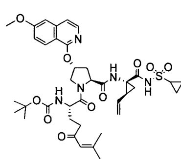
I-96
