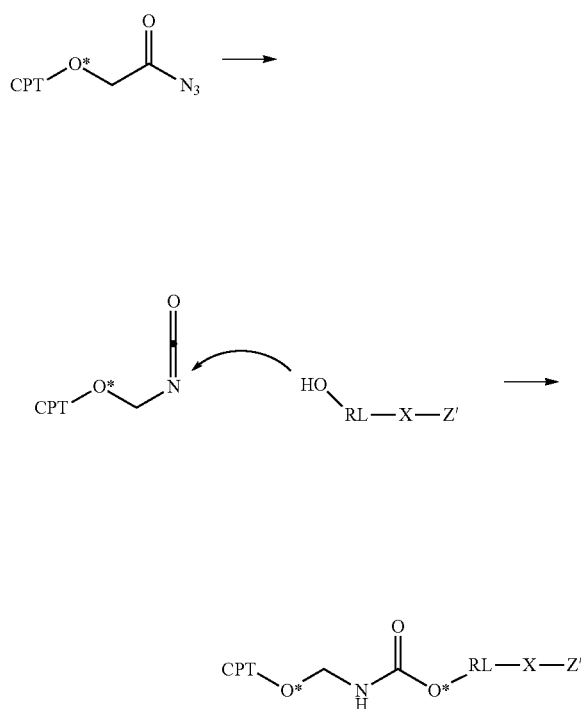
Scheme 2: Preparation of Exemplary Camptothecin Drug-Linker compounds of formula Z'-A-RL-Y-D , Z'-A-S^*-RL-Y-D or Z'-A-B(S^*)-RL-Y-D wherein Y has formula (a') using the Curtius Rearrangement Reaction
