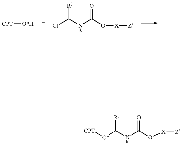
Scheme 3: Alternative preparation of exemplary Camptothecin Drug-Linker compounds of formula Z'-A-RL-Y-D , Z'-A-S^*-RL-Y-D or Z'-A-B(S^*)-RL-Y-D wherein Spacer Unit Y is a methylene carbamate unit of formula (a) or formula (a') via N-chloromethylamine synthesis
