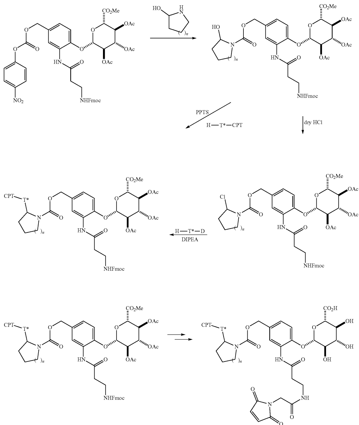
Scheme 4: Preparation of exemplary Camptothecin Drug-Linker compounds of formula Z' - A - RL - Y - D wherein Spacer Unit Y is a formula (a'') methylene carbamate unit.
