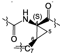
C7 syn to carbonyl
