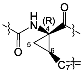
C7 syn to carbonyl
