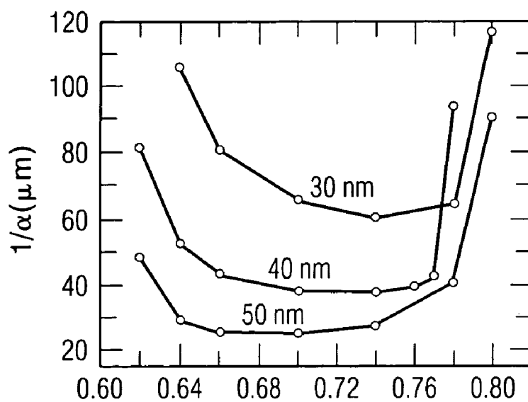
FIG. 20 THICKNESS OF CLADDING LAYER( \mu\text{m} )
