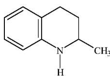
2-methyl-1,2,3,4-tetrahydroquinoline
