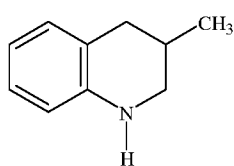
3-methyl-1,2,3,4-tetrahydroquinoline
