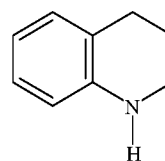
1,2,3,4-tetrahydroquinoline
