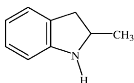
2-methylindoline
