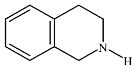
1,2,3,4-tetrahydroisoquinoline
