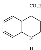
1,2,3,4-tetrahydroquinoline-4-carboxylic acid
