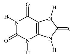
Uric acid
