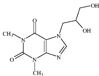
Dyphylline
