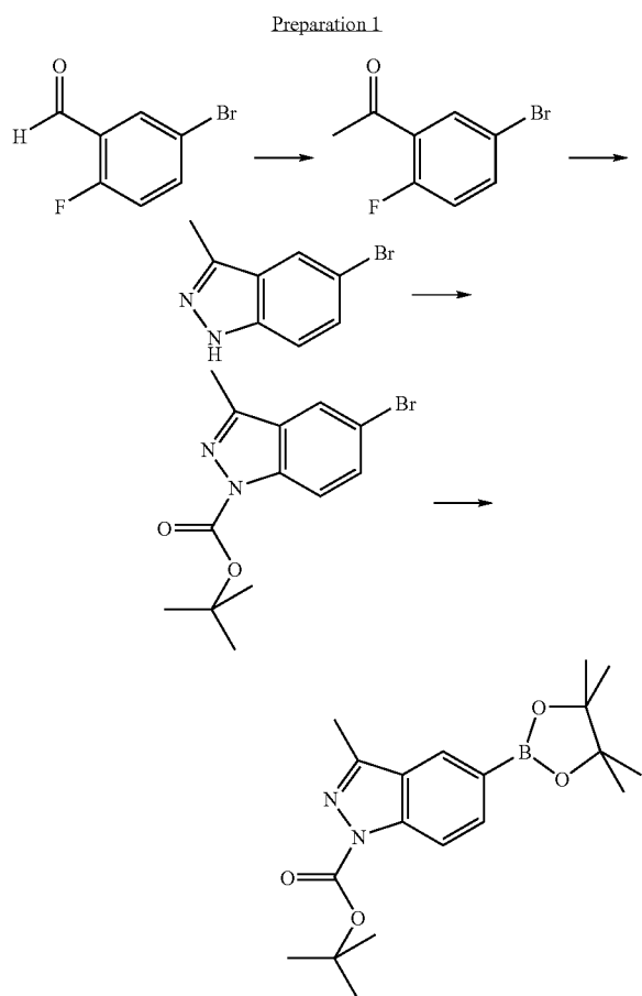
Preparation 1. Preparation of 3-Methyl-5-(4,4,5,5-tetramethyl-1,3,2-dioxaborolan-2-yl)-indazole-1-carboxylic acid tert-butyl ester
