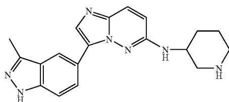
3-(3-methyl-1H-indazol-5-yl)-N-piperidin-3-yl-imidazo[1,2-b]pyridazin-6-amine
