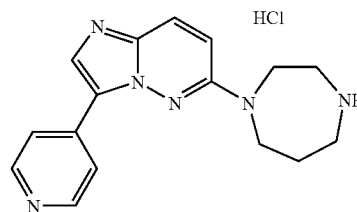
6-(1,4-diazepan-1-yl)-3-pyridin-4-yl-imidazo[1,2-b]pyridazine
