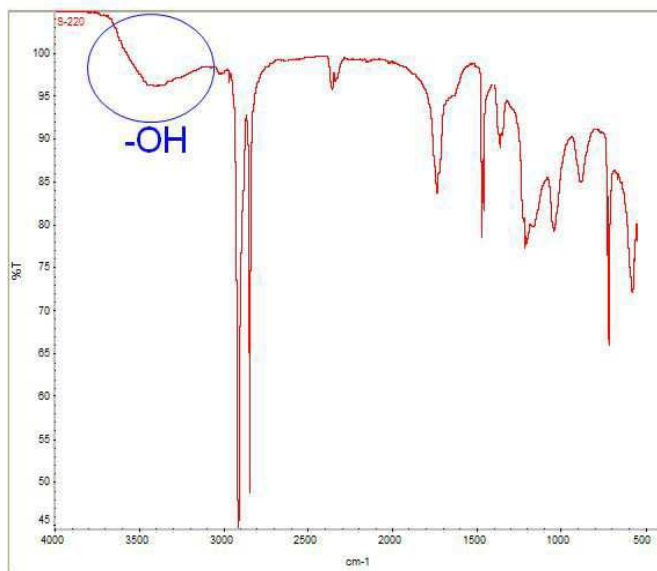
Sulfonated S-20 separator
