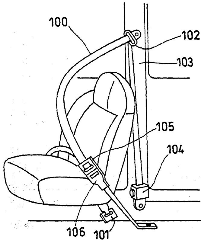
FIG.15 (RELATED ART)
