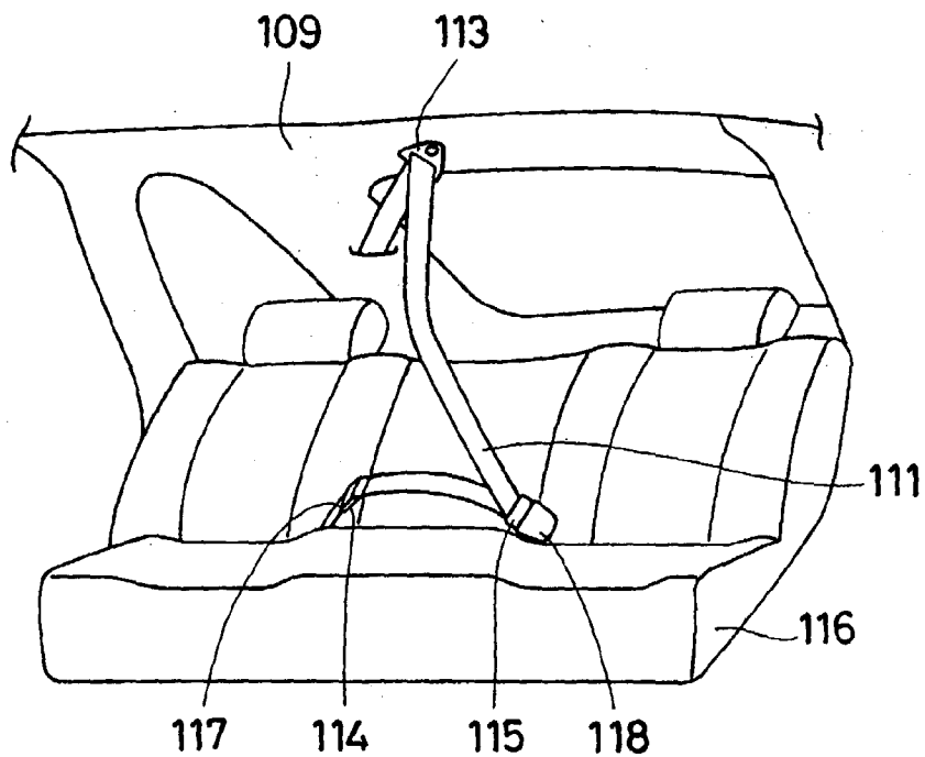
FIG.16 (RELATED ART)
