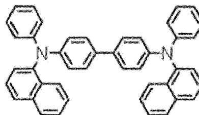
NPD
