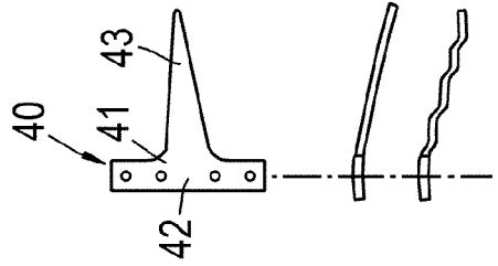
Fig.5c Repeat Axial Cross Section (tang only)
