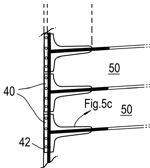
Fig.5b View on A
