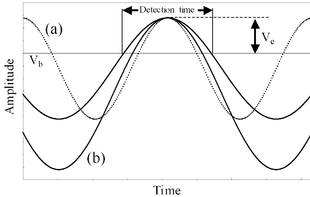
Variation of the detection time due to the changes of the gate (a) frequency and (b) amplitude
