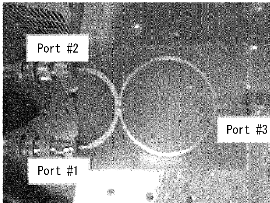
(c) 500MHz band-3dB-Wilkinson power coupler
