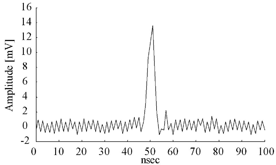
Output signal with BRF
