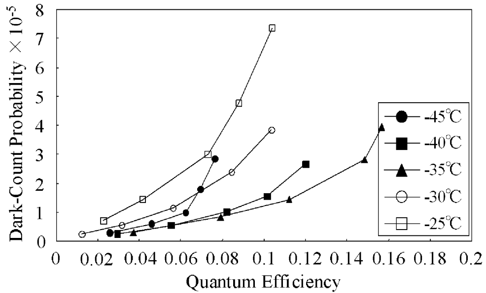
(b) Quantum efficiency vs. dark-count probability at different temperature
