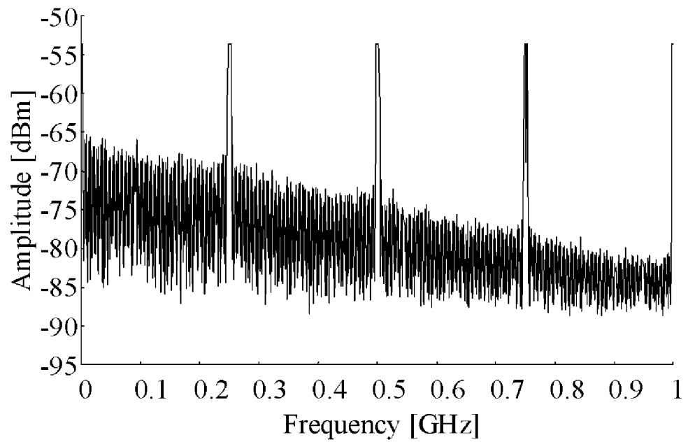
(b) excess bias voltage 4.2V
