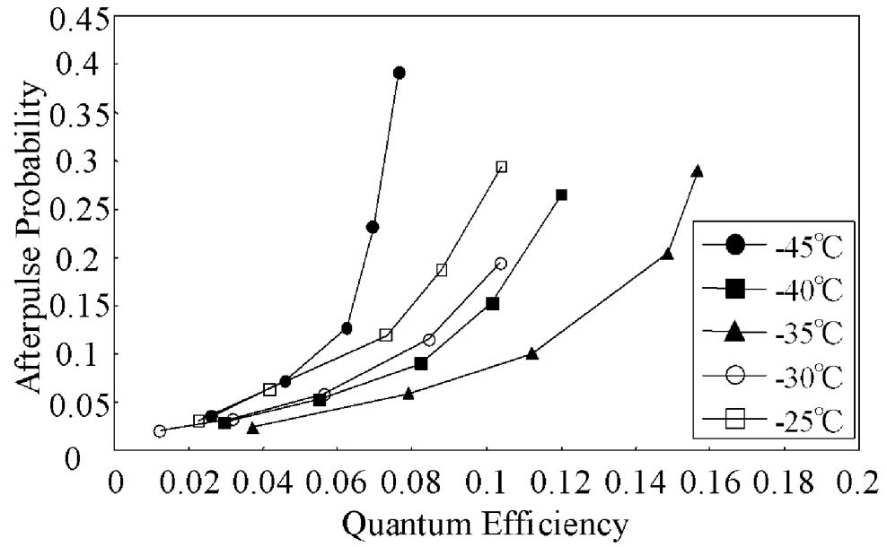
(a) Quantum efficiency vs. afterpulse probability at different temperature
