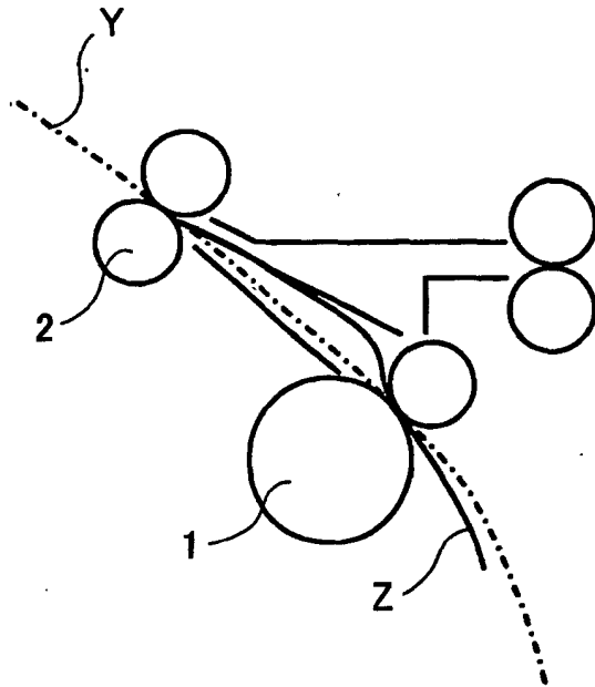
FIG. 1 PRIOR ART
