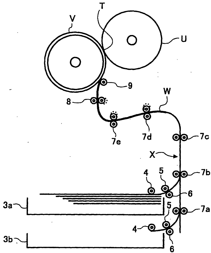
FIG. 3 PRIOR ART
