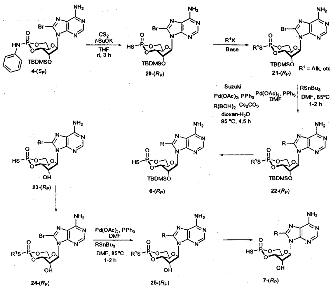
Scheme 10
