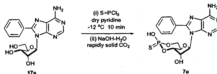
Scheme 5
