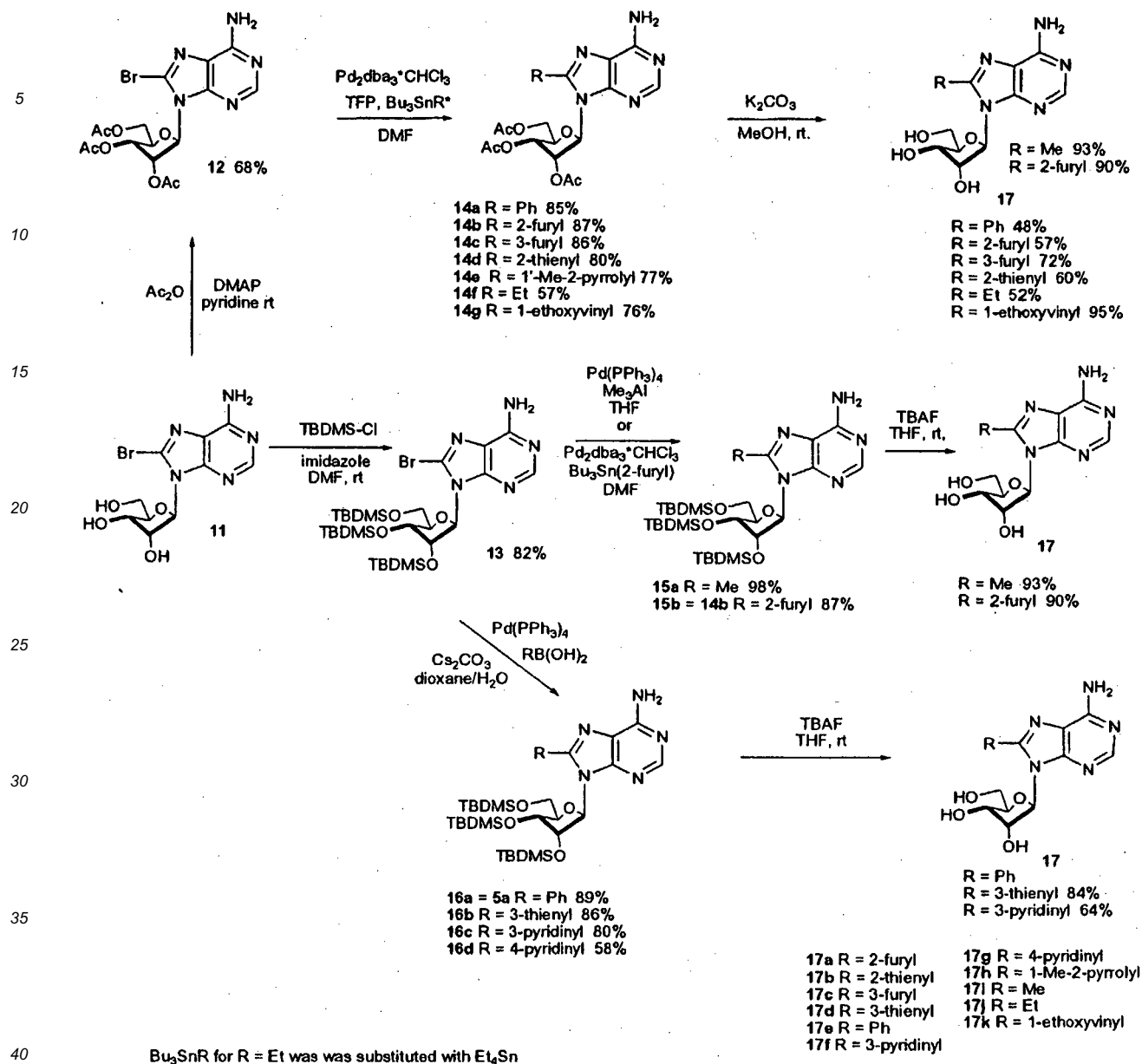
Scheme 7
