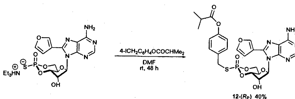
Scheme 2b
