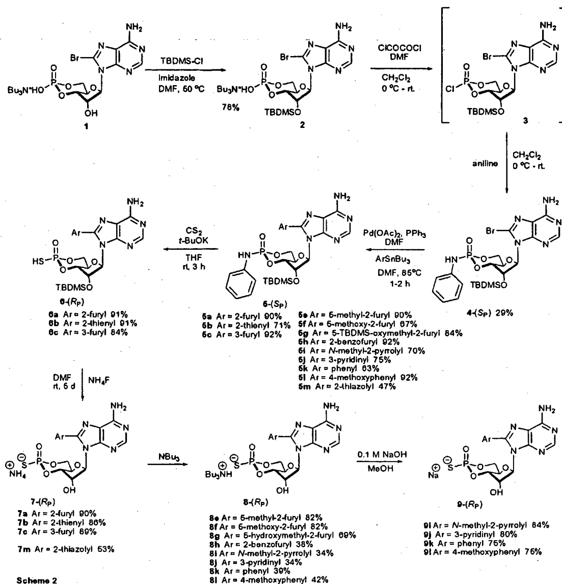
Scheme 2
