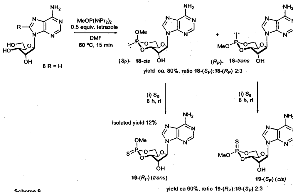
Scheme 9
