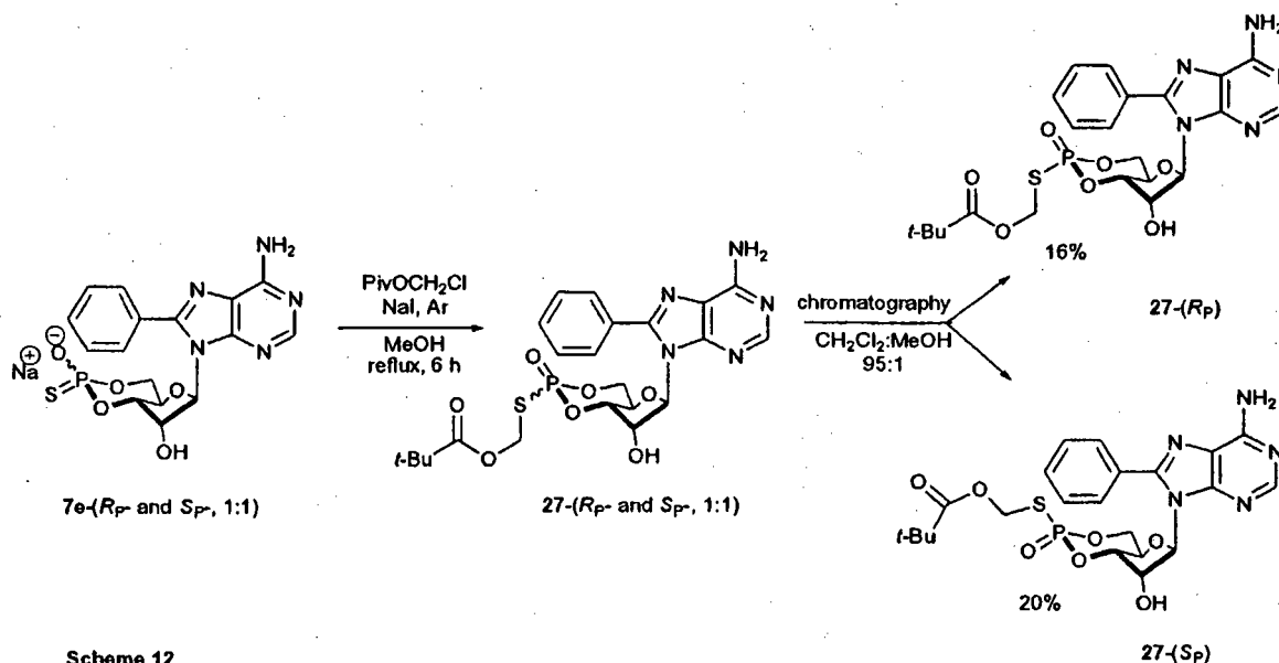
Scheme 12
