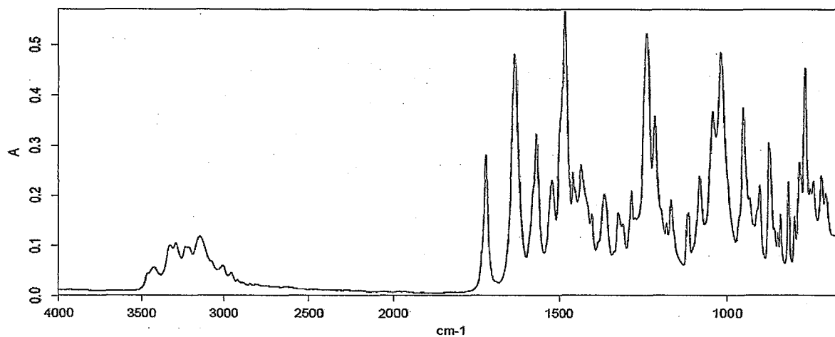
Di-DMSO solvate
