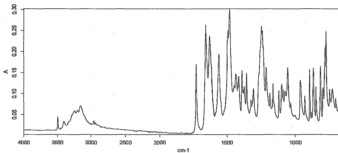
DMF/water solvate
