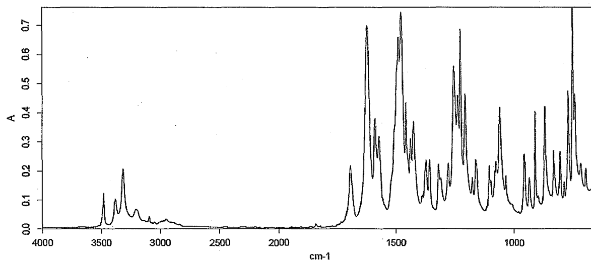
Polymorph III
