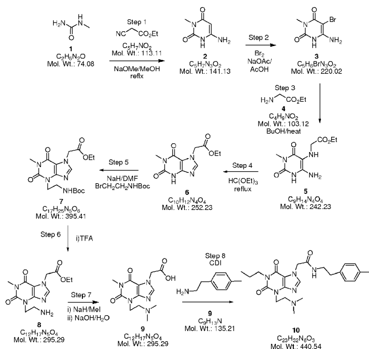
Scheme 12
