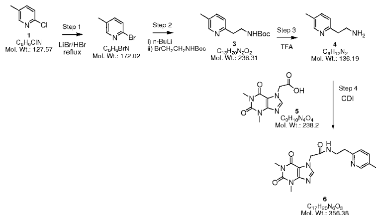
Scheme 15
