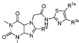
formula (VIIIb)
