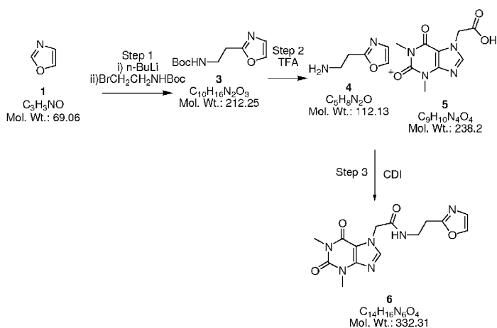
Scheme 11
