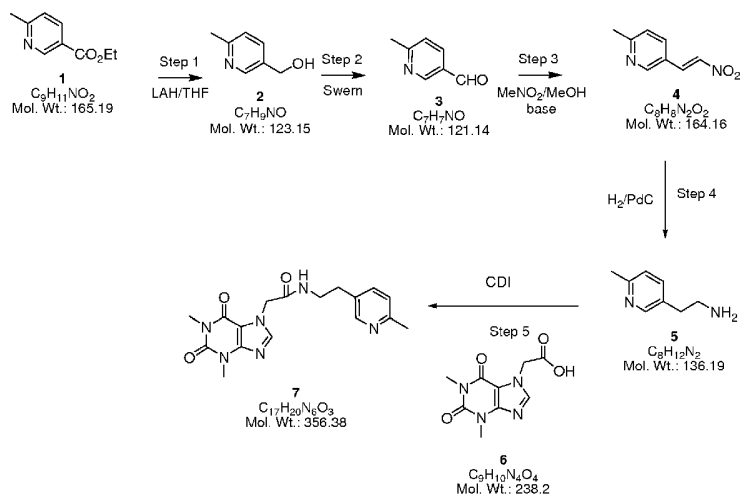
Scheme 16
