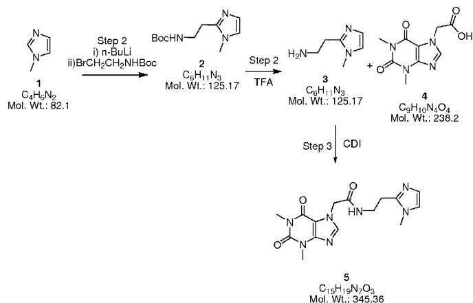
Scheme 9
