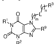
Formula (Ic)
