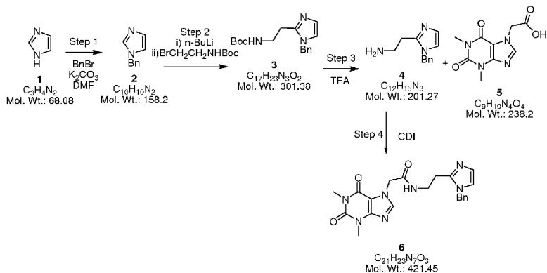
Scheme 8
