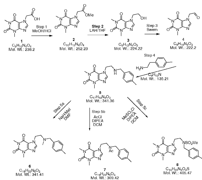
Scheme 5
