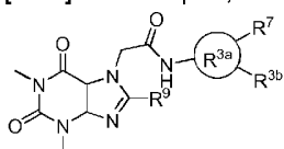
formula (VIIIa)
