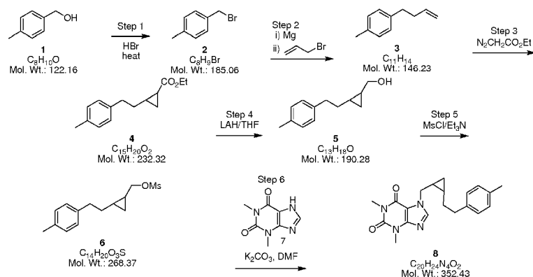
Scheme 14
