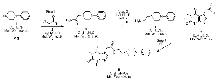
Scheme 7
