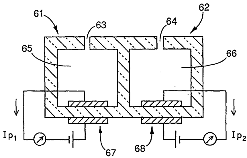
FIG. 25 PRIOR ART
