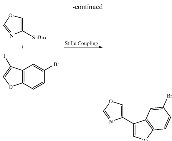
Stille Coupling No. 2
