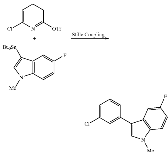
Stille Coupling No. 3
