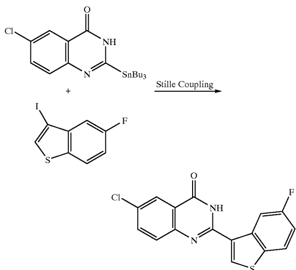
Stille Coupling No. 3
