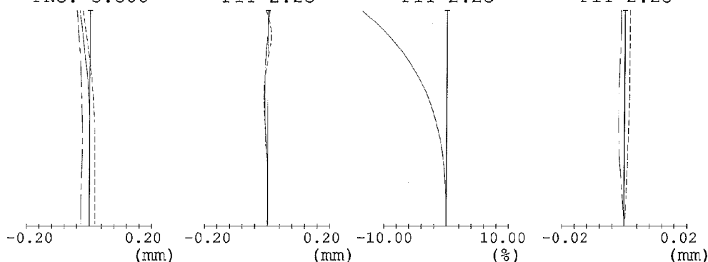
FIG. 35E FIG. 35F FIG. 35G FIG. 35H SPHERICAL CHROMATIC ABERRATION ABERRATION OF FNO. 4.729 FIY 2.25 FIY 2.25 FIY 2.25
