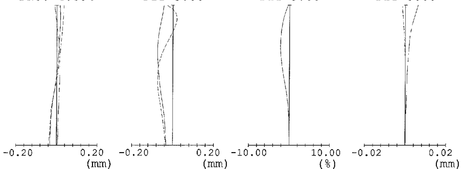
FIG.10I FIG.10J FIG.10K FIG.10L SPHERICAL CHROMATIC ABERRATION ABERRATION OF FNO. 5.200 FIY 3.00 FIY 3.00 FIY 3.00 MAGNIFICATION
