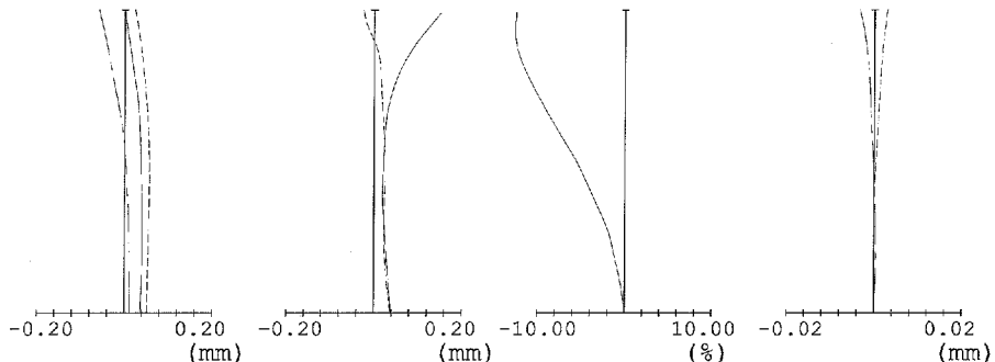
FIG.10E FIG.10F FIG.10G FIG.10H SPHERICAL CHROMATIC ABERRATION ABERRATION OF FNO. 4.396 FIY 3.00 FIY 3.00 FIY 3.00 MAGNIFICATION
