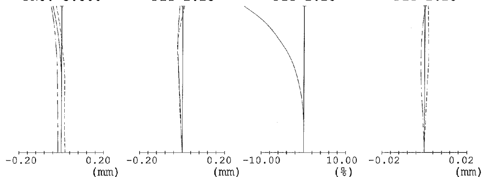
FIG. 38E FIG. 38F FIG. 38G FIG. 38H SPHERICAL CHROMATIC ABERRATION ABERRATION OF FNO. 4.662 FIY 2.25 FIY 2.25 FIY 2.25
