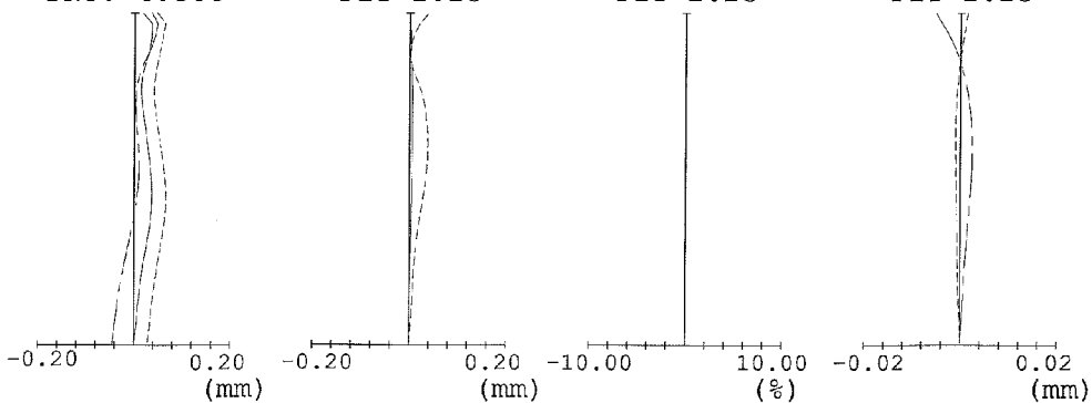
FIG. 38I FIG. 38J FIG. 38K FIG. 38L SPHERICAL CHROMATIC ABERRATION ABERRATION OF FNO. 4.800 FIY 2.25 FIY 2.25 FIY 2.25
