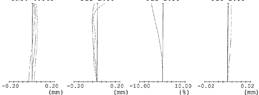
FIG. 23E FIG. 23F FIG. 23G FIG. 23H SPHERICAL CHROMATIC ABERRATION ABERRATION OF FNO. 4.511 FIY 2.99 FIY 2.99 FIY 2.99
