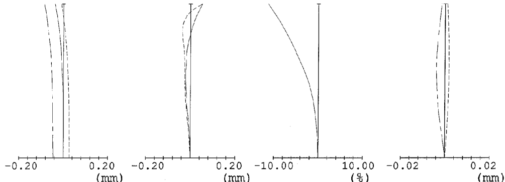
FIG. 41E FIG. 41F FIG. 41G FIG. 41H SPHERICAL ABERRATION ASTIGMATISM DISTORTION CHROMATIC FNO. 3.726 FIY 2.99 FIY 2.99 ABERRATION OF MAGNIFICATION FIY 2.99
