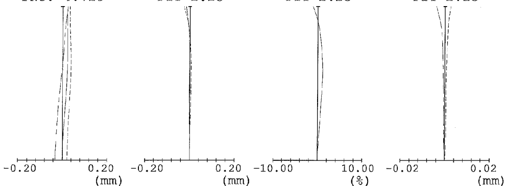
FIG. 35I FIG. 35J FIG. 35K FIG. 35L SPHERICAL CHROMATIC ABERRATION ABERRATION OF FNO. 4.800 FIY 2.25 FIY 2.25 FIY 2.25
