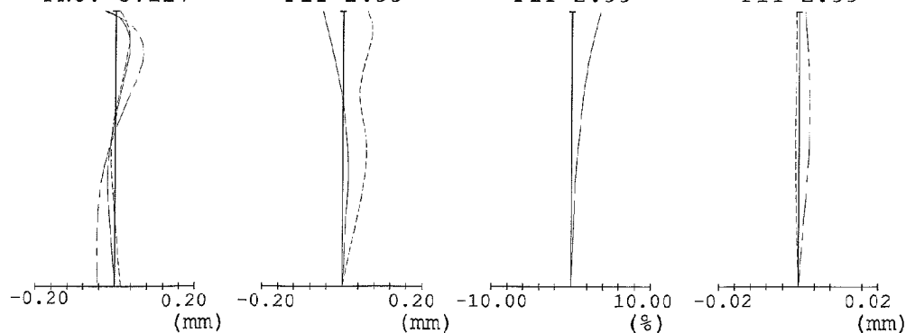
FIG. 23I FIG. 23J FIG. 23K FIG. 23L SPHERICAL CHROMATIC ABERRATION ABERRATION OF FNO. 5.127 FIY 2.99 FIY 2.99 FIY 2.99
