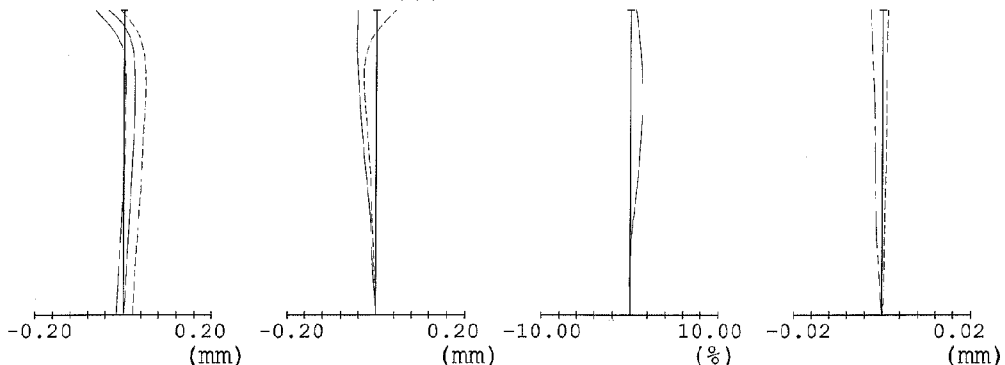
FIG. 41I FIG. 41J FIG. 41K FIG. 41L SPHERICAL ABERRATION ASTIGMATISM DISTORTION CHROMATIC FNO. 5.123 FIY 2.99 FIY 2.99 ABERRATION OF MAGNIFICATION FIY 2.99
