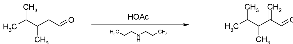
3,4-dimethyl-pentanal
