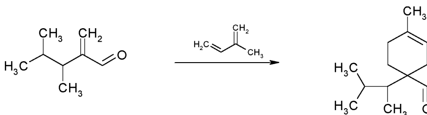
1-(1,2-dimethyl-propyl)-4-methyl-cyclohex-3-enecarbaldehyde
