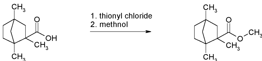
1,2,4-trimethyl-bicyclo[2.2.1]heptane-2-carboxylic acid
