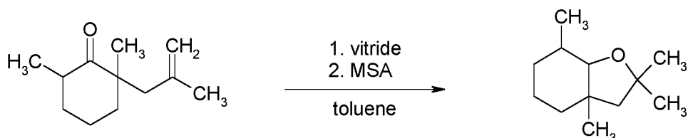
2,6-dimethyl-2-(2-methyl- allyl)-cyclohexanone
