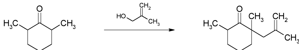
2,6-dimethyl- cyclohexanone
