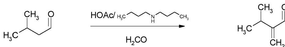
3-methyl-butyraldehyde
