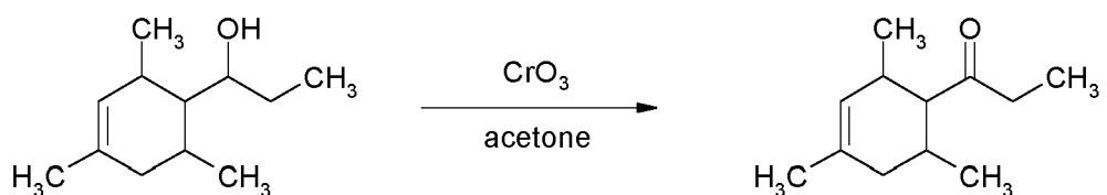
1-(2,4,6-trimethyl-cyclohex-3-enyl)-propan-1-ol
