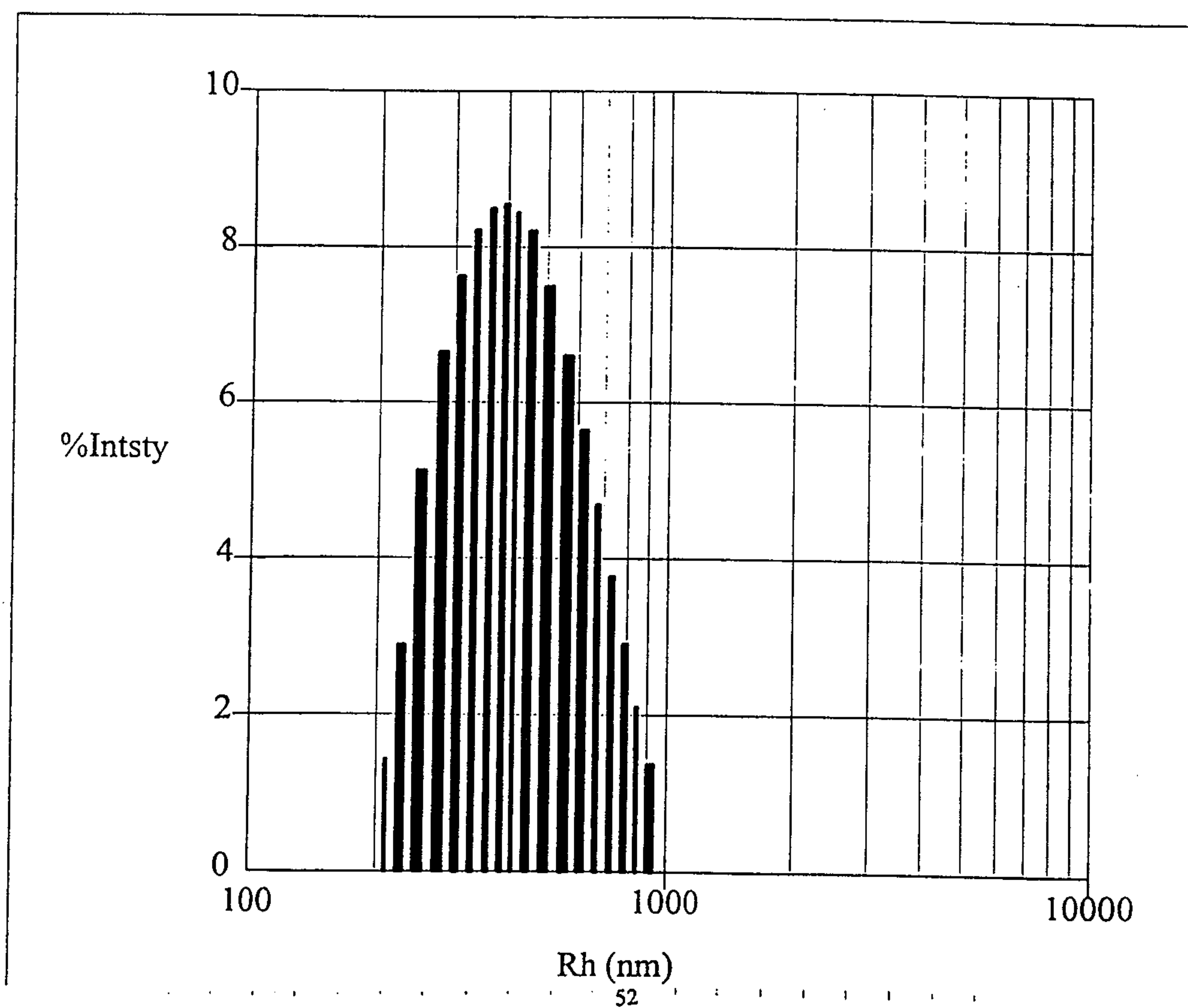
Regularization Histogram
