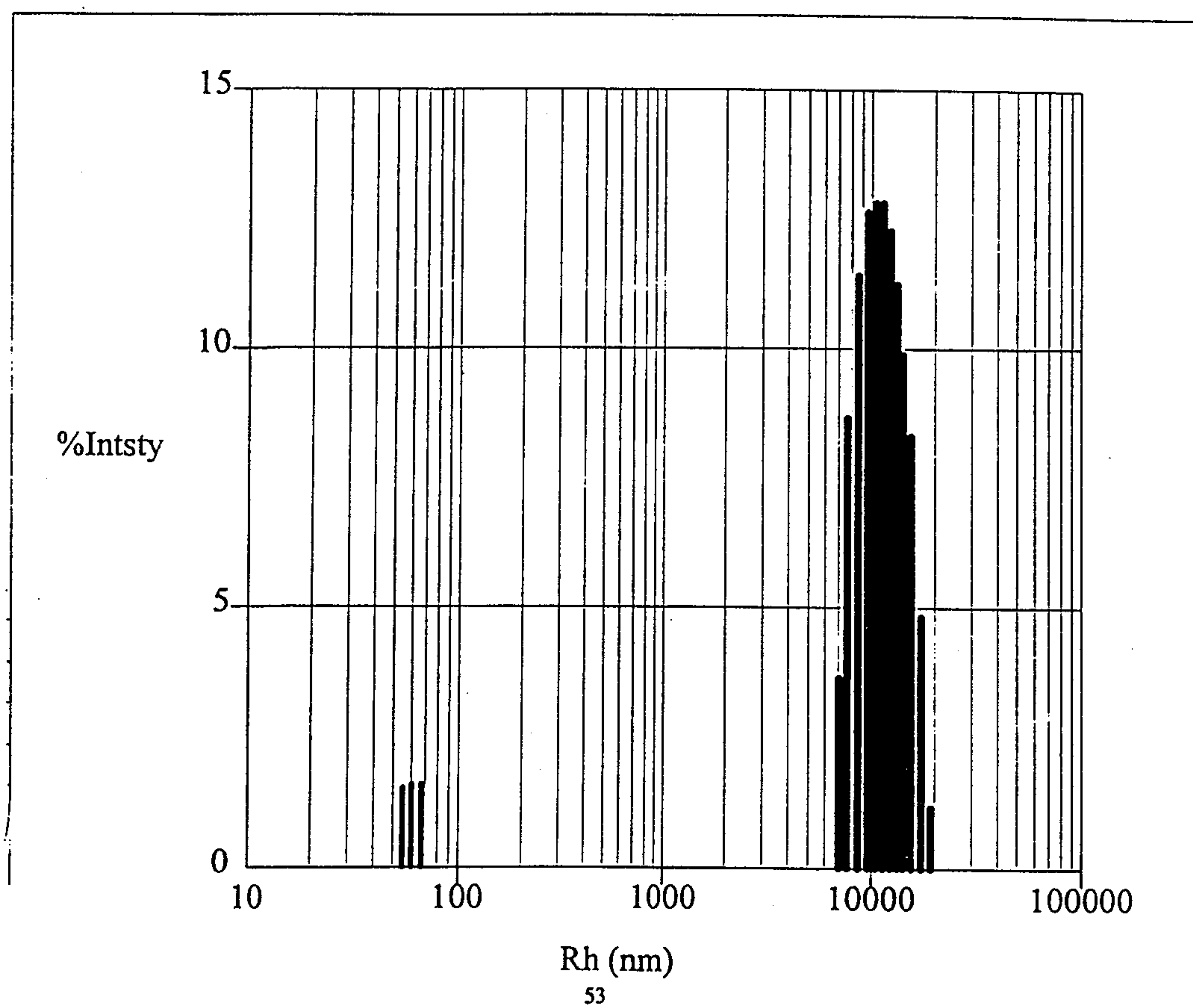
Regularization Histogram
