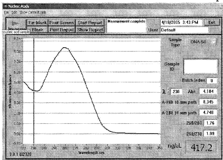
Figure 2C. Concentration sample 1
