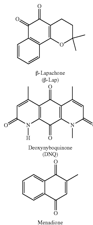
Scheme 1. Examples of Quinone Compounds.
