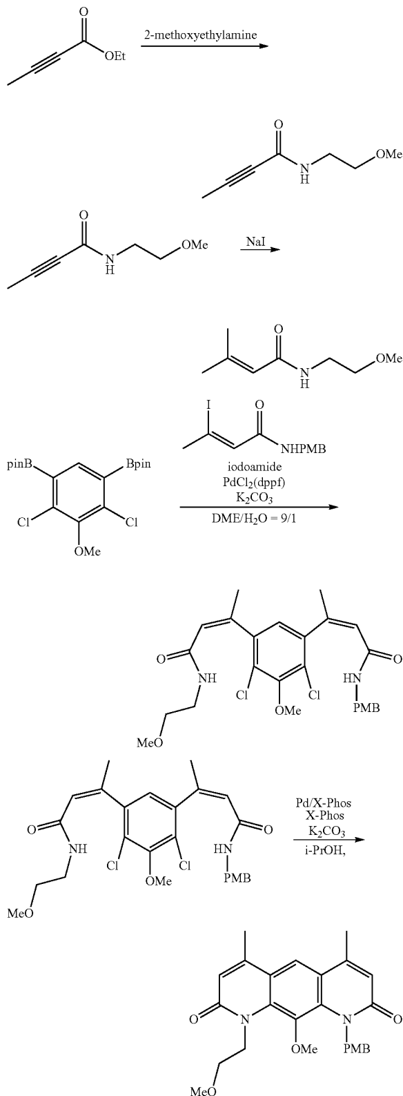
Scheme 7.4. Preparation of DNQ-P4.
