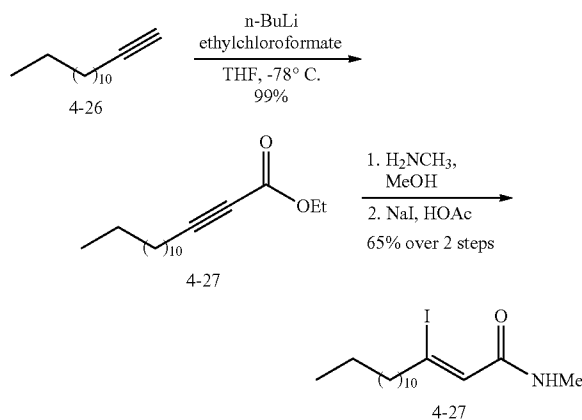
Scheme 4.2. Synthesis of alkynes 4-19 and 4-21 for preparation of 4-10 and 4-13.
