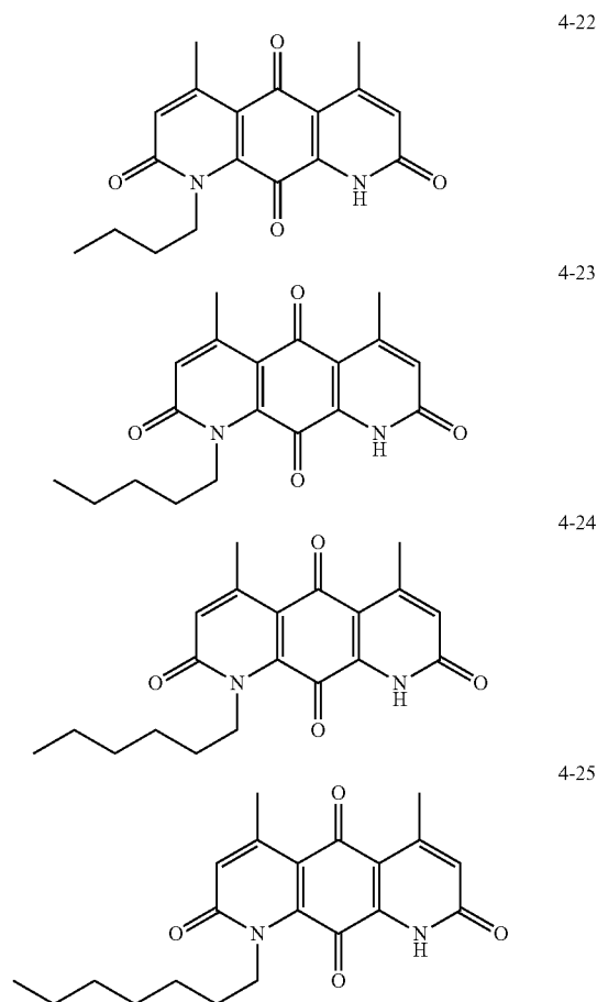
Scheme 4.3. New DNQ derivatives.
