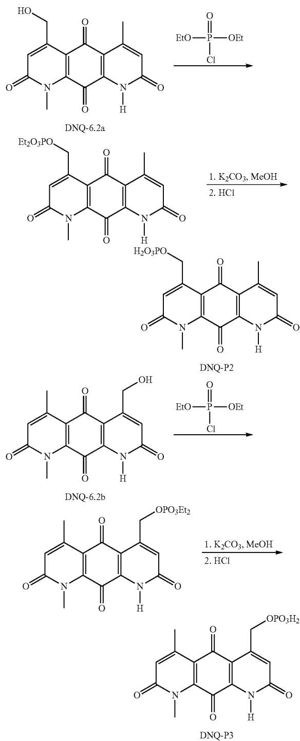
Scheme 7.3. Preparation of DNQ-P2 and DNQ-P3.
