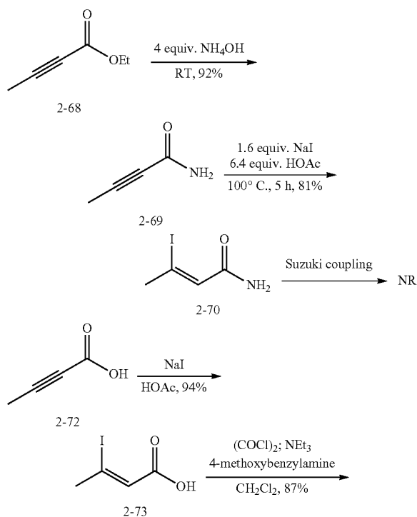
Scheme 1.13. Synthesis of DNQ by methylation of 2-67.
