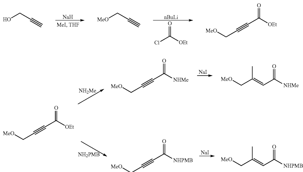
Scheme 7.2. Preparation of DNQ-P2 and DNQ-P3 Intermediates.
