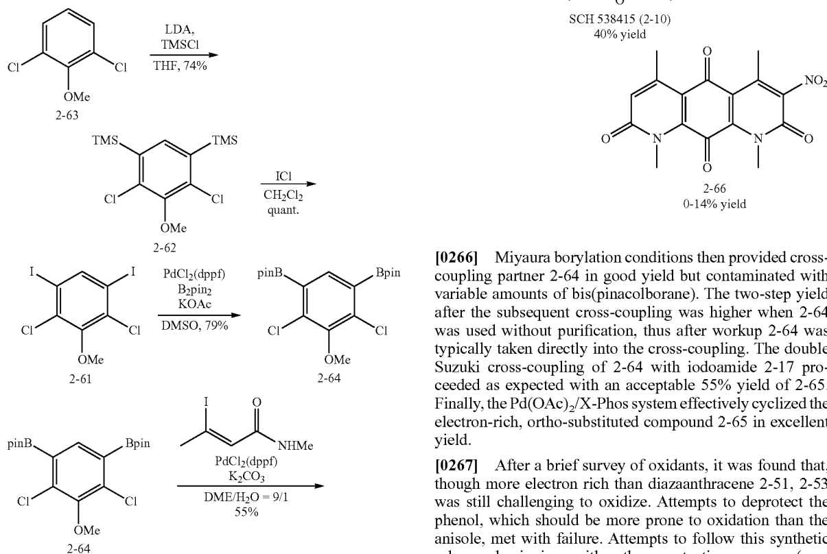
Scheme 1.12. Synthesis of SCH 538415.
