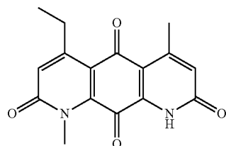
4.1 Scheme 4.1. Nine DNQ derivatives.
