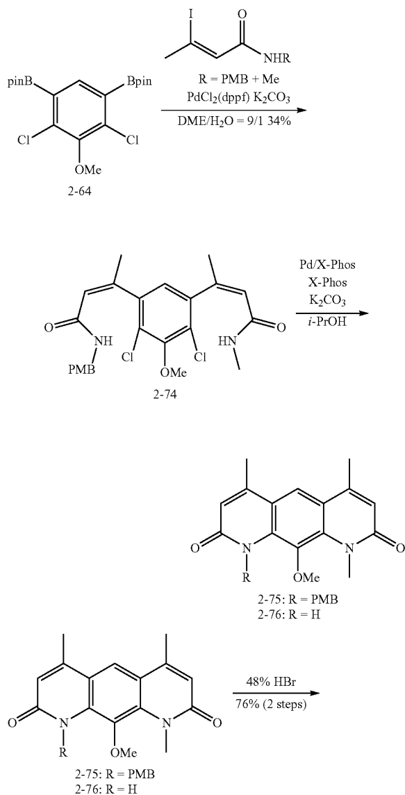
Scheme 1.14. Robust and scalable synthesis of DNQ.
