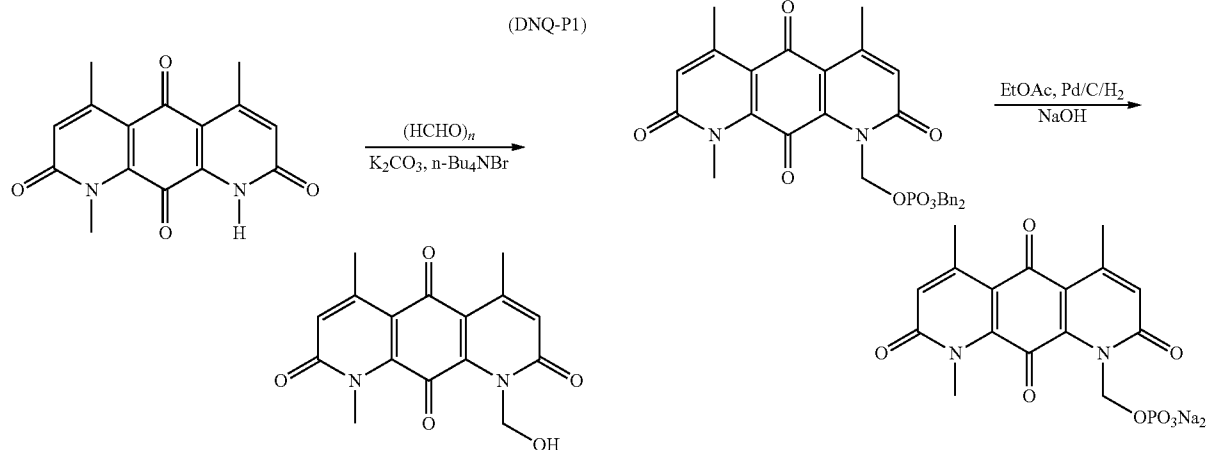
Scheme 7.1. Preparation of DNQ-P1.
