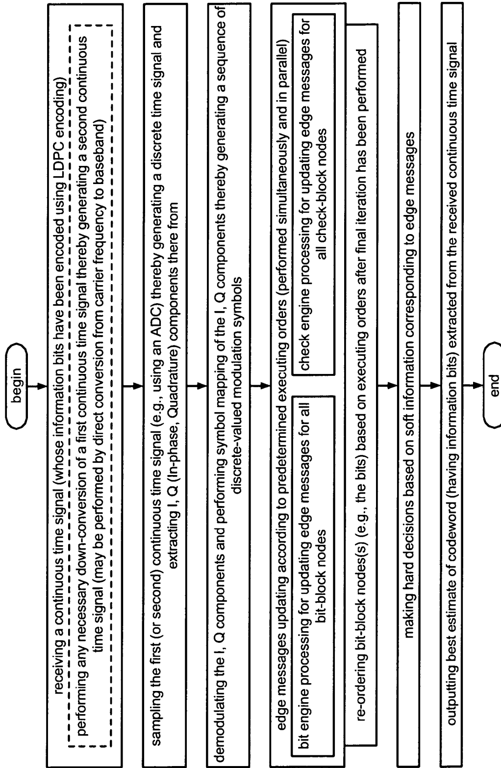
method for performing LDPC bit-check parallel decoding
