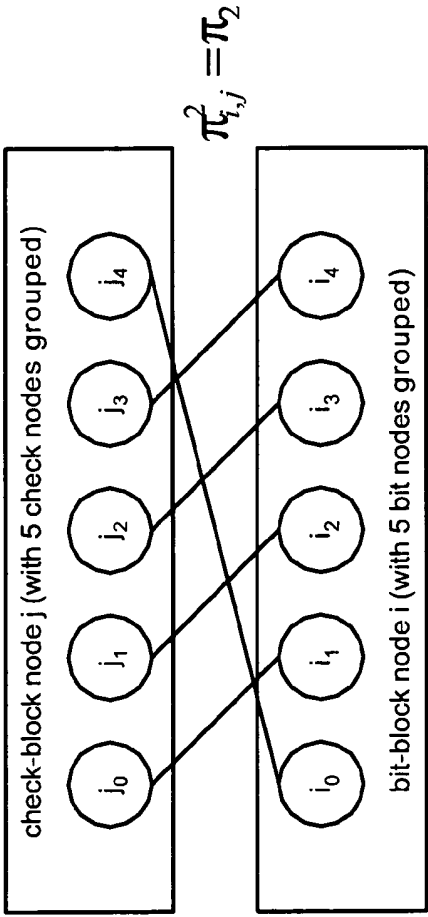
example of permutation, \pi_{i,j}^2 , providing linkage between LDPC block bipartite graph and LDPC bipartite graph Fig. 31B
