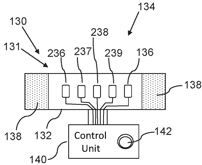
Trigger Device
