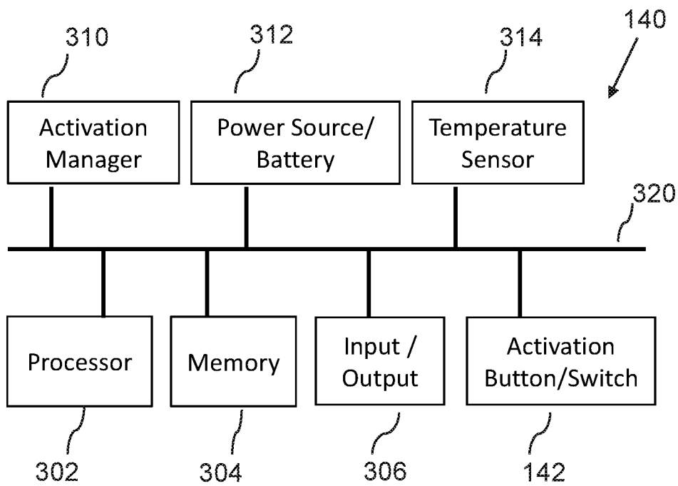
Control Unit
