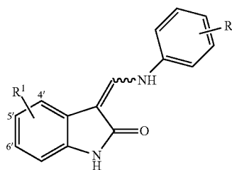
R 1 R Substitution 2 3 4 5 6 Unsubstituted, 4-Fluoro, 4-methyl, 5-Chloro, 5-Fluoro, & 6-Fluoro 3-[(Substitued Phenylamino)-methylene]-1,3-dihydro-indol-2-ones.
