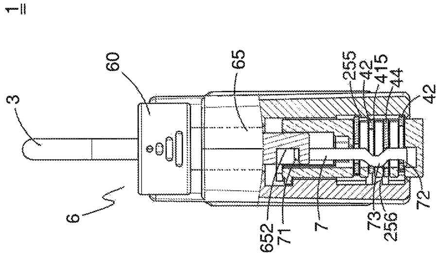
B-B cross-section
