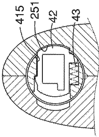
C-C cross-section
