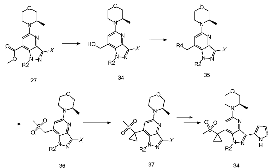
Scheme 7: Alternative synthesis route to cyclopropyl azaindazole derivatives
