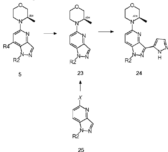
Scheme 5: Synthesis route to azaindazole 24
