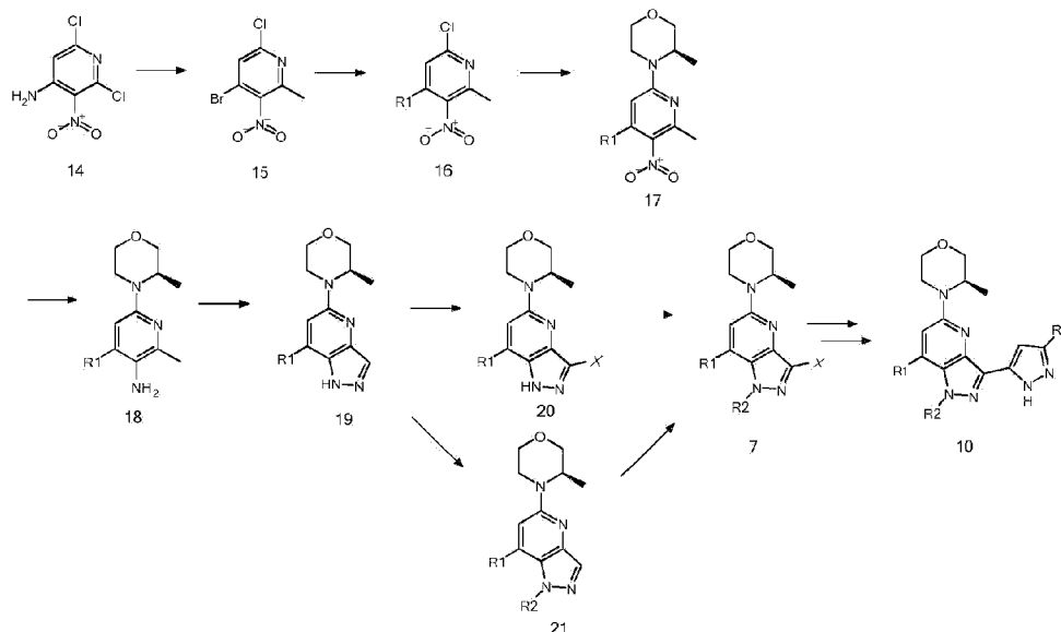
Scheme 3: Alternative synthesis route to Azaindazole 10
