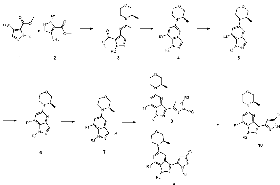
Scheme 1: Synthesis route to azaindazole 10
