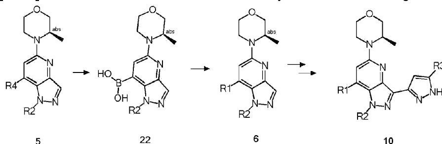
Scheme 4: Alternative Suzuki type reaction to azaindazole 6 and subsequently to 10 .
