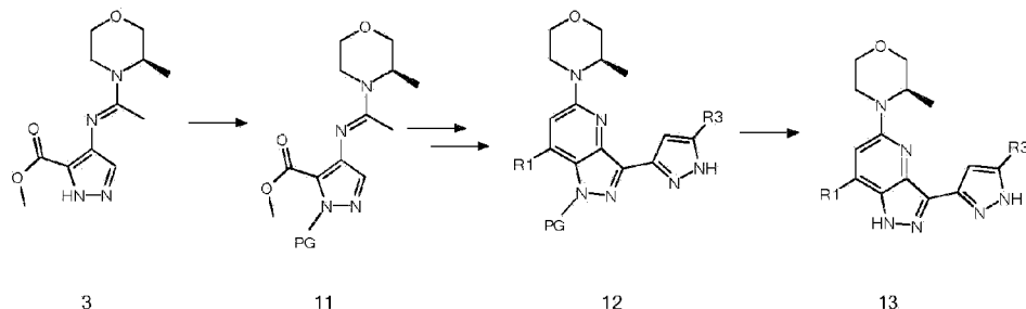
Scheme 2: Synthesis route to unsubstituted azaindazole 13
