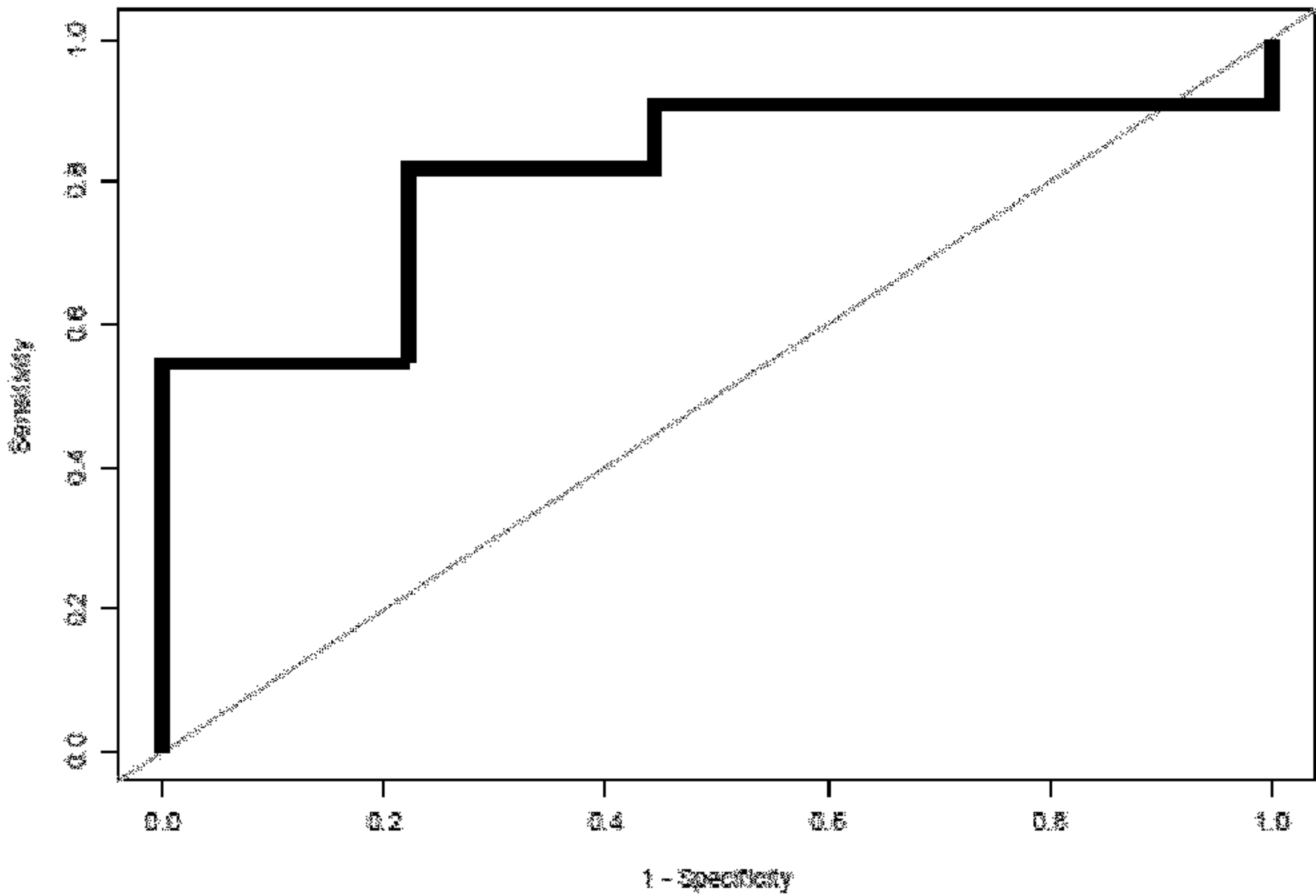
ROC-Curve:
