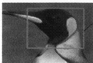
ORIGINAL IMAGE
