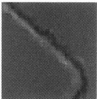
NEAREST NEIGHBOR
