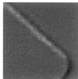
MARKOV CHAIN
