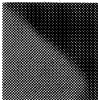
LOW-FREQUENCY IMAGE
