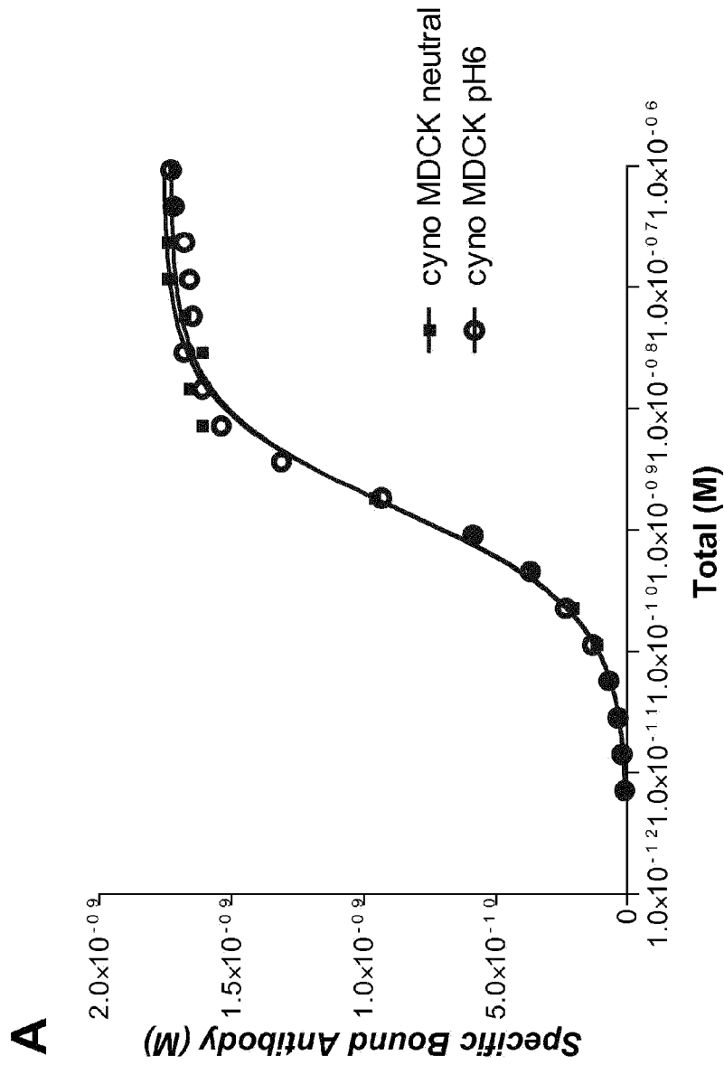
FIGURE 6A- CA170_01519.g57 Fab' binding on cynomolgus MDCK II (cm) cells in acidic and neutral pH
