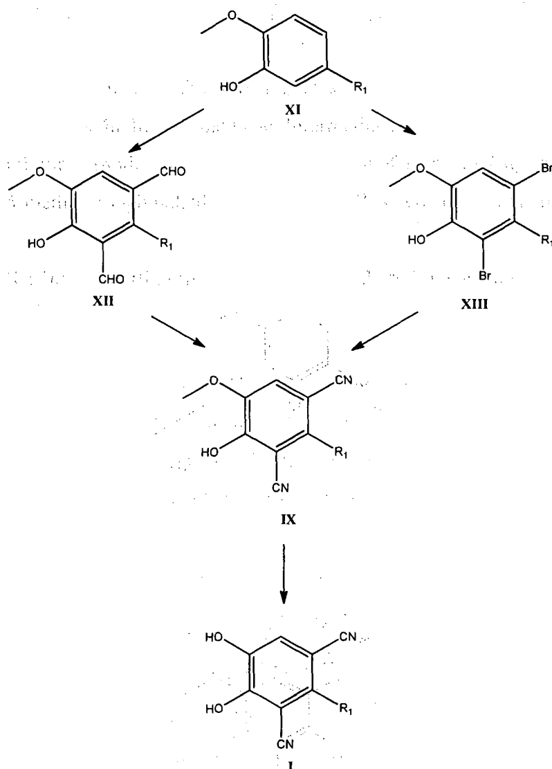
Scheme 3. Starting from a 5-substituted 2-methoxyphenol
