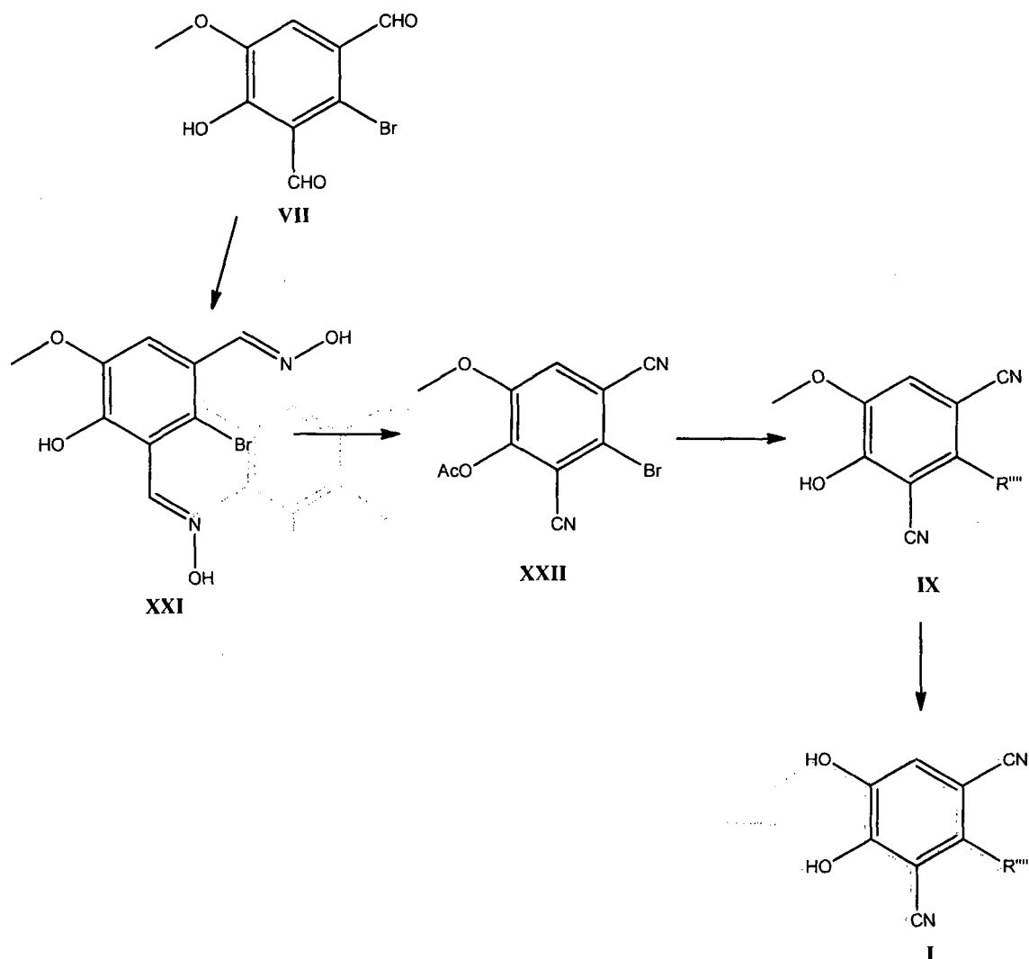
Scheme 5. Conversion of 2-bromo-4-hydroxy-5-methoxyisophthalaldehyde
