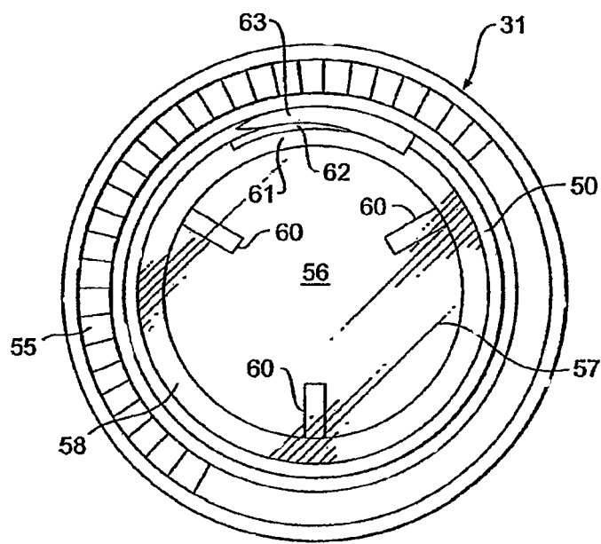
FIG. 3 PRIOR ART
