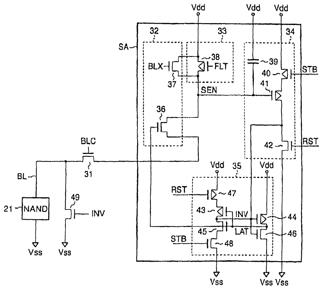
FIG. 8 PRIOR ART
