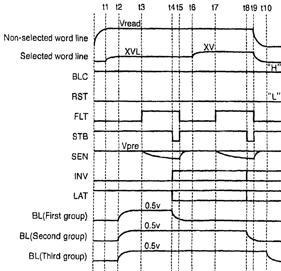
FIG. 9 PRIOR ART
