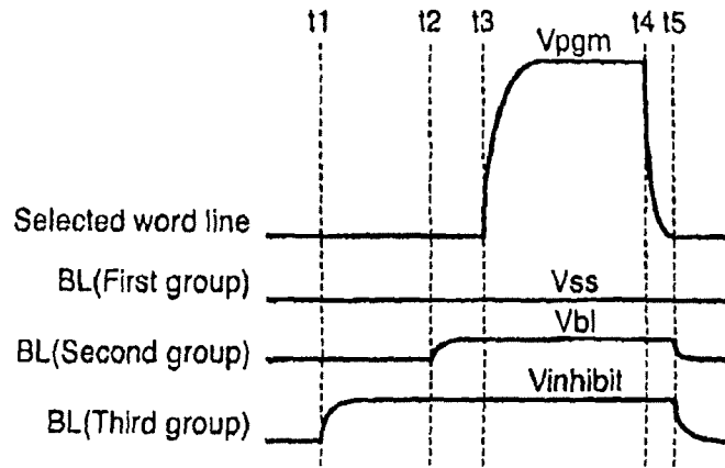
FIG. 12 PRIOR ART
