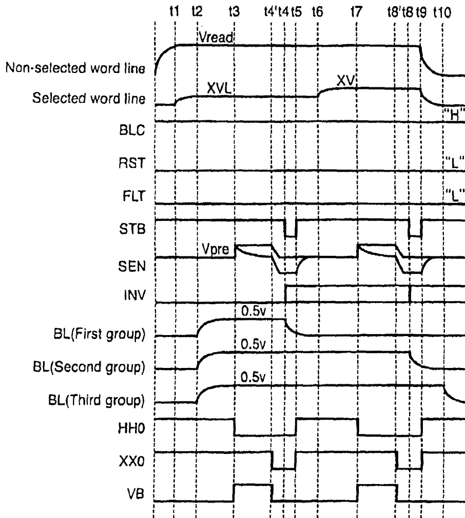
FIG. 11 PRIOR ART
