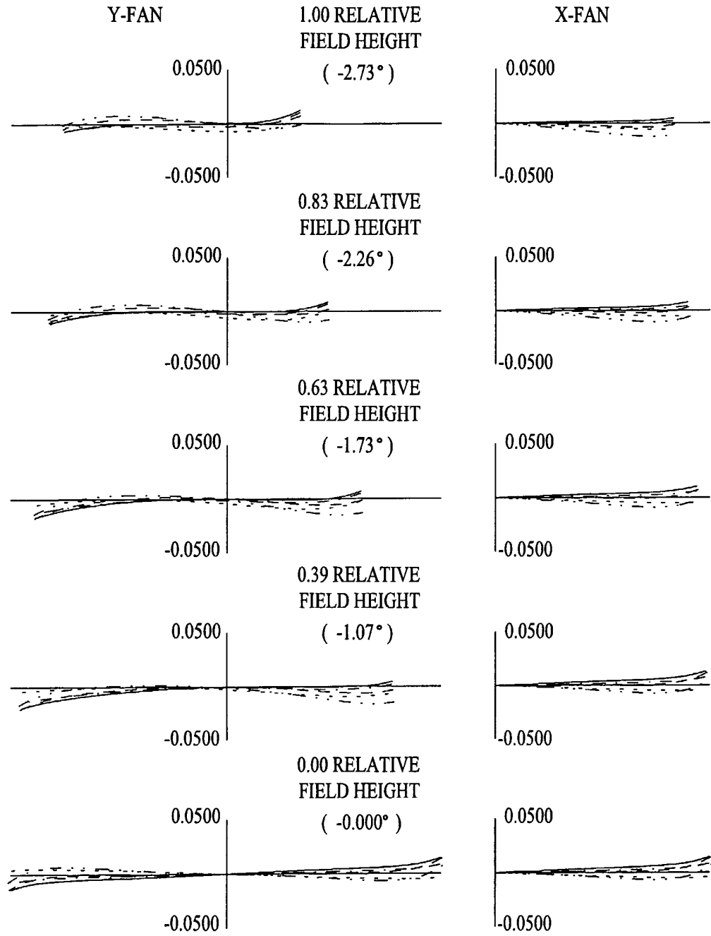
Fig. 57 RAY ABERRATIONS ( MILLIMETERS ) ----- 643.8469 NM ----- 587.5600 NM POSITION 19 ----- 546.0700 NM ----- 486.1300 NM ----- 460.0000 NM
