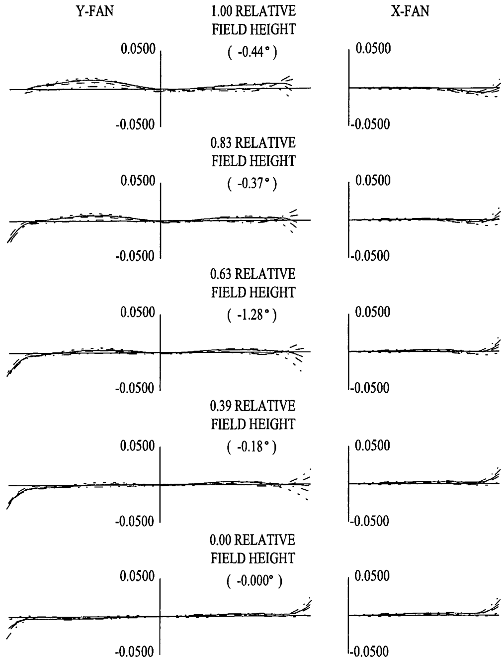
Fig. 49 RAY ABERRATIONS ( MILLIMETERS ) ----- 643.8469 NM ----- 587.5600 NM POSITION 11 ----- 546.0700 NM ----- 486.1300 NM ----- 460.0000 NM
