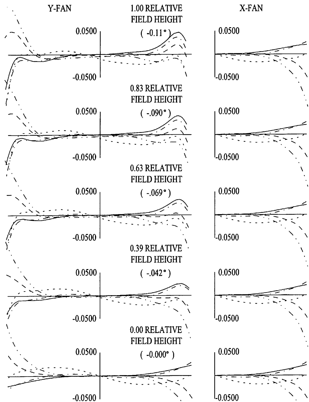
Fig. 52 RAY ABERRATIONS ( MILLIMETERS ) POSITION 14
