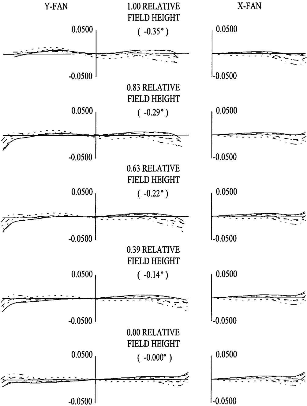
Fig. 54 RAY ABERRATIONS ( MILLIMETERS ) POSITION 16 ----- 643.8469 NM ----- 587.5600 NM ----- 546.0700 NM ----- 486.1300 NM ----- 460.0000 NM
