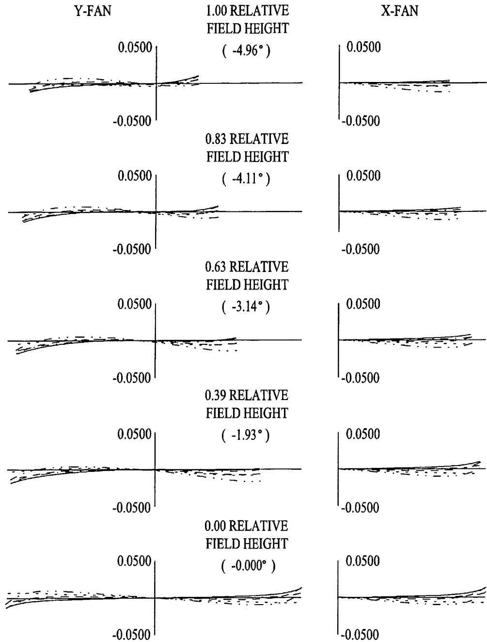
Fig. 44 RAY ABERRATIONS ( MILLIMETERS ) POSITION 6 ----- 643.8469 NM ----- 587.5600 NM ----- 546.0700 NM ----- 486.1300 NM ----- 460.0000 NM
