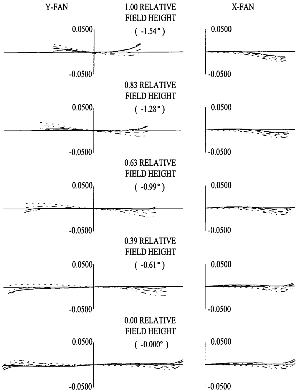
Fig. 47 RAY ABERRATIONS ( MILLIMETERS ) POSITION 9 ----- 643.8469 NM ----- 587.5600 NM ----- 546.0700 NM ----- 486.1300 NM ----- 460.0000 NM
