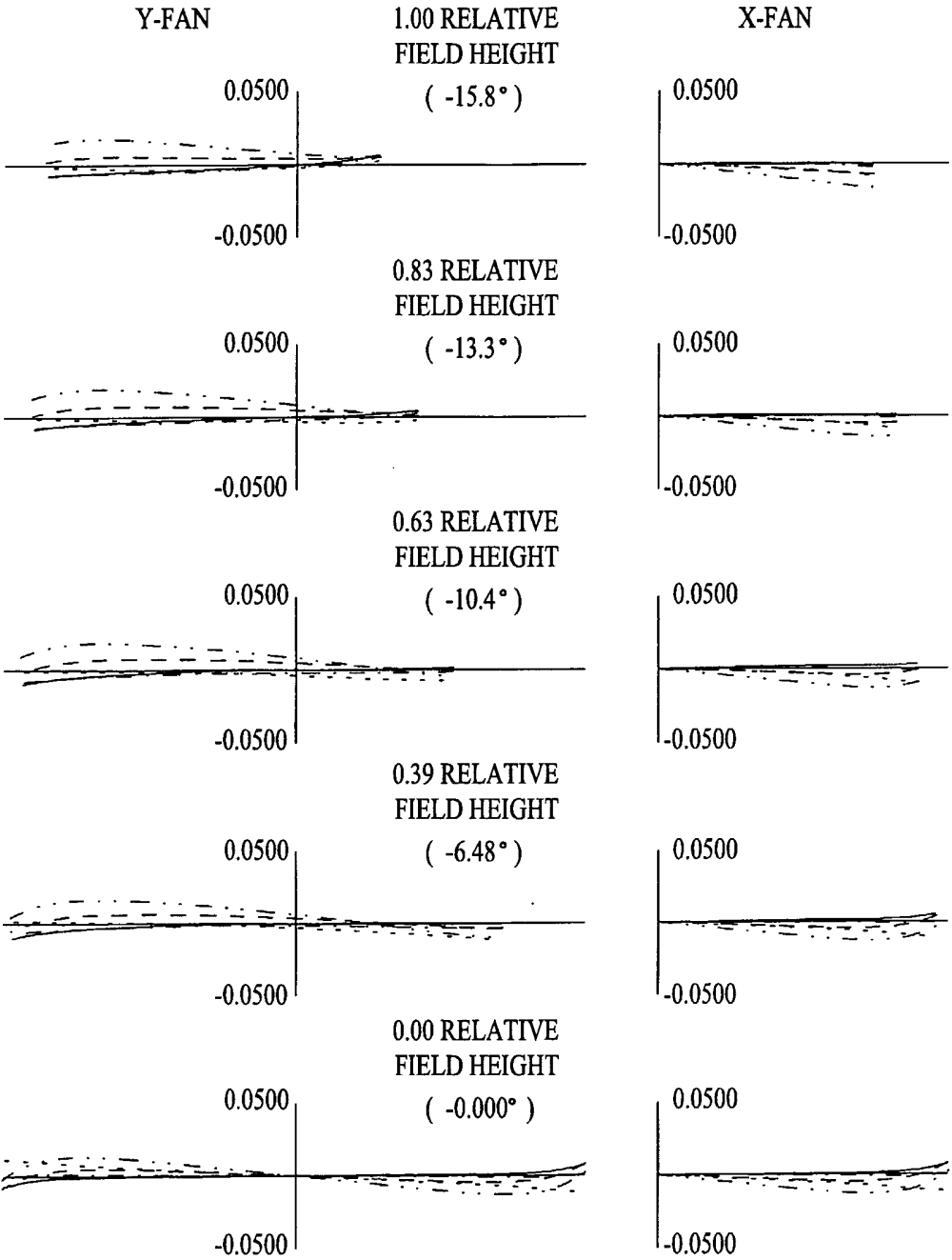
Fig. 42 RAY ABERRATIONS ( MILLIMETERS ) POSITION 4 ----- 643.8469 NM ----- 587.5600 NM ----- 546.0700 NM ----- 486.1300 NM ----- 460.0000 NM
