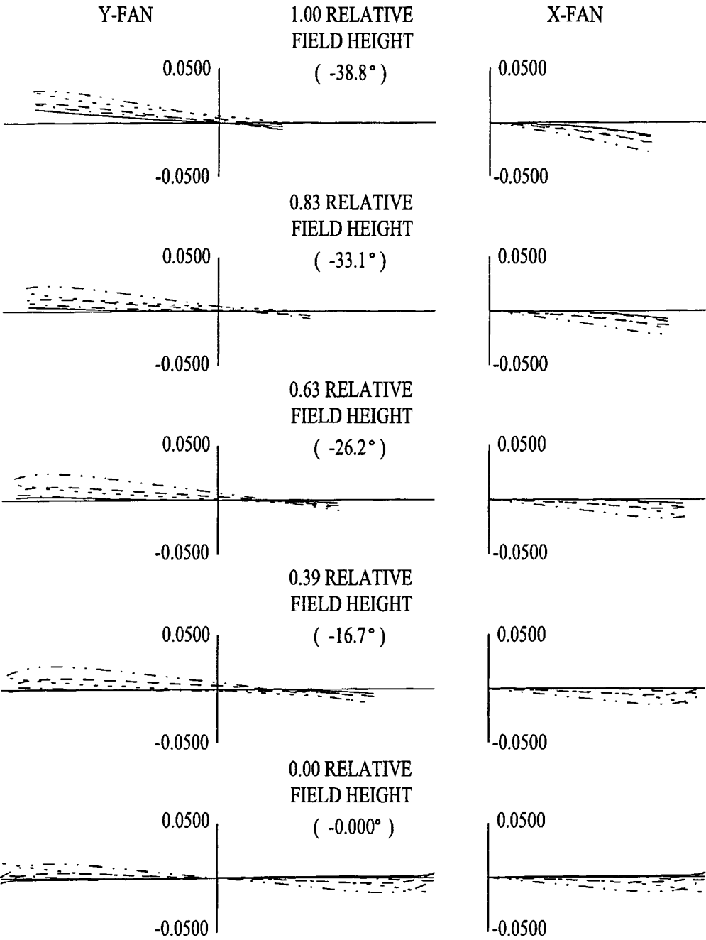
Fig. 39 RAY ABERRATIONS (MILLIMETERS) POSITION 1 ----- 643.8469 NM ----- 587.5600 NM ----- 546.0700 NM ----- 486.1300 NM ----- 460.0000 NM
