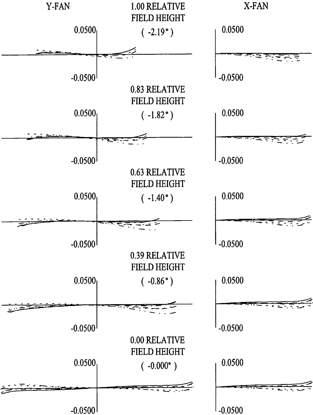
Fig. 46 RAY ABERRATIONS ( MILLIMETERS ) POSITION 8 ----- 643.8469 NM ----- 587.5600 NM ----- 546.0700 NM ----- 486.1300 NM ----- 460.0000 NM
