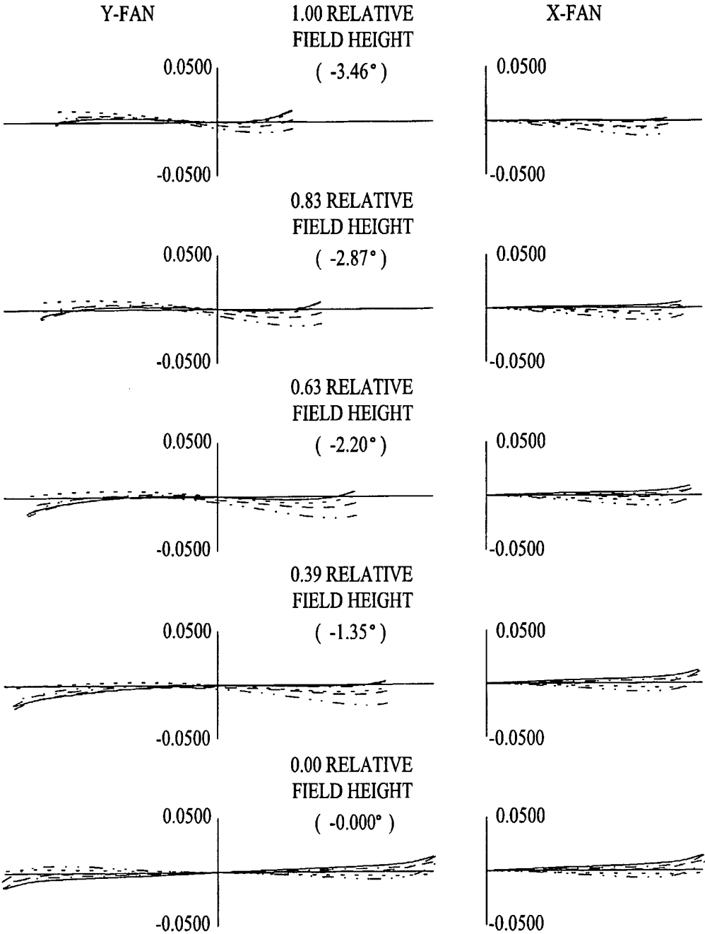
Fig. 45 RAY ABERRATIONS ( MILLIMETERS ) POSITION 7 ----- 643.8469 NM - - - - - 587.5600 NM ————— 546.0700 NM - - - - - 486.1300 NM .-.-.-.- 460.0000 NM
