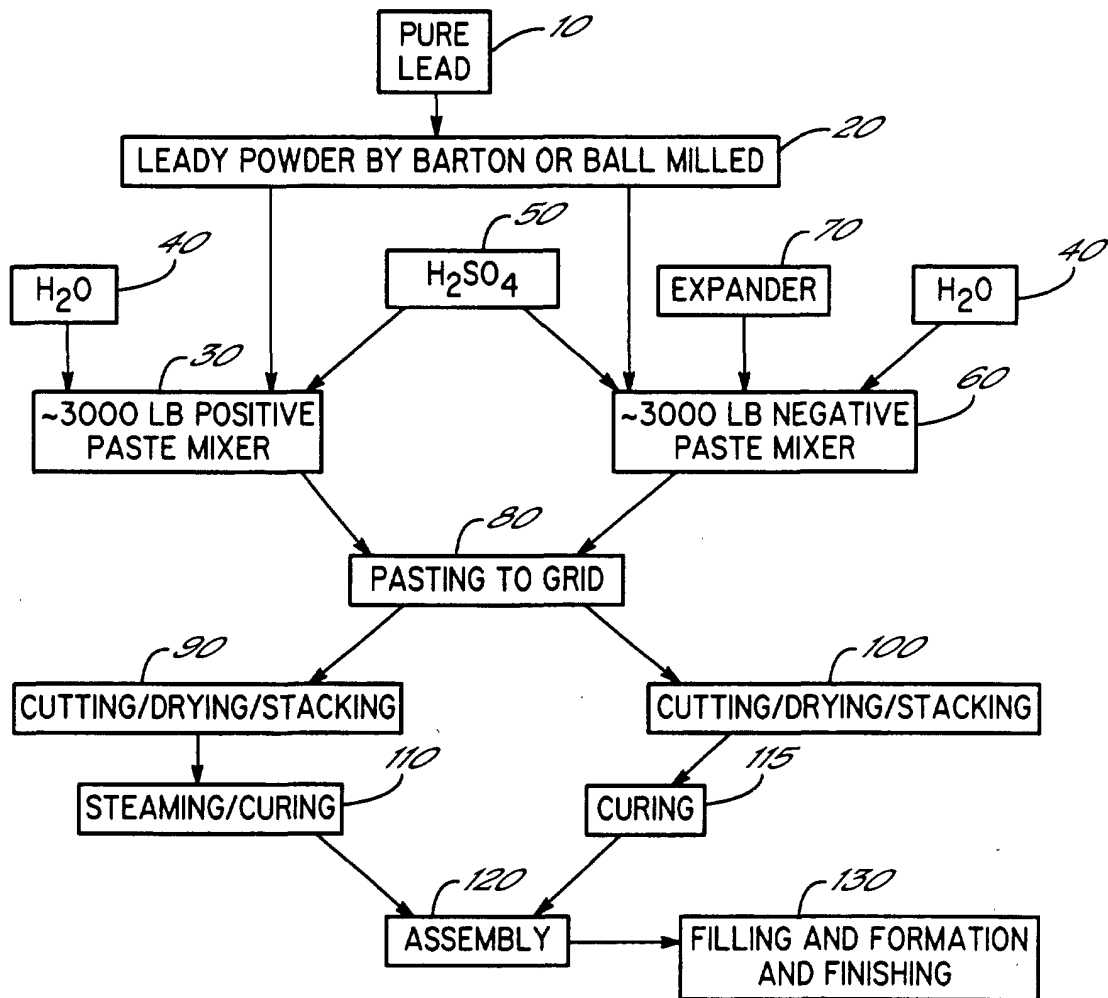
Fig.1. PRIOR ART
