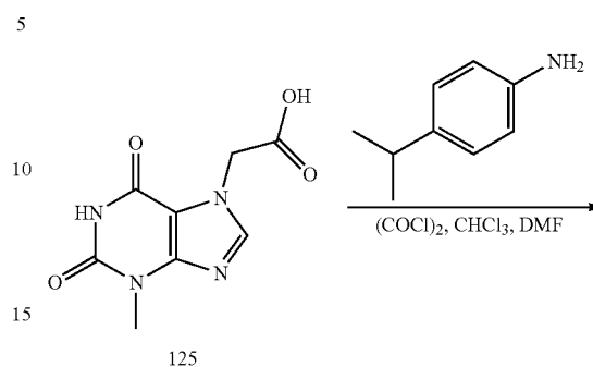
N-(4-isopropylphenyl)-2-(3-methyl-2,6-dioxo-1,2,3,6-tetrahydropurin-7-yl)acetamide (388)
