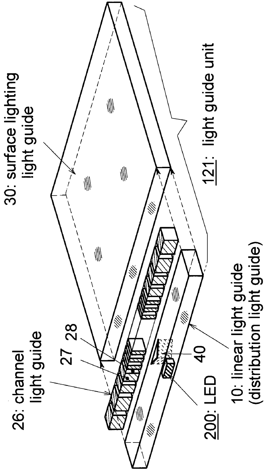
FIG. 25 SURFACE LIGHT SOURCE
