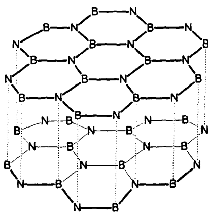
\alpha -Bornitrid
