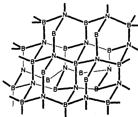
\beta -Bornitrid
