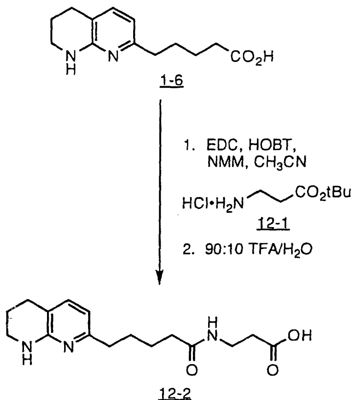
3-(5-(5,6,7,8-Tetrahydro-[1,8]naphthyridin-2-yl)-pentanoylamino)-propionic acid (12-2)
