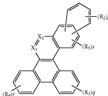
[Chemical Formula 7]
