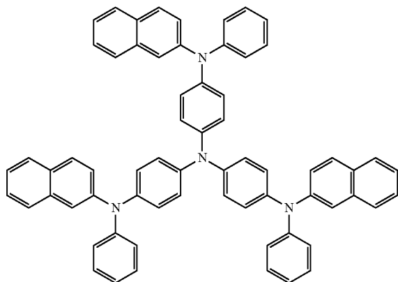
2-TNATA
