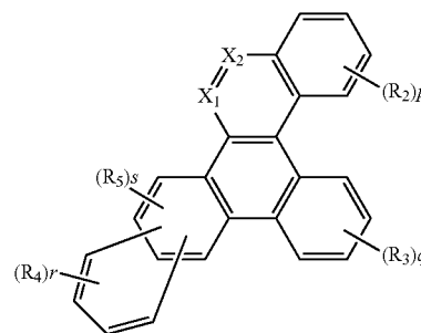
[Chemical Formula 8-1]
