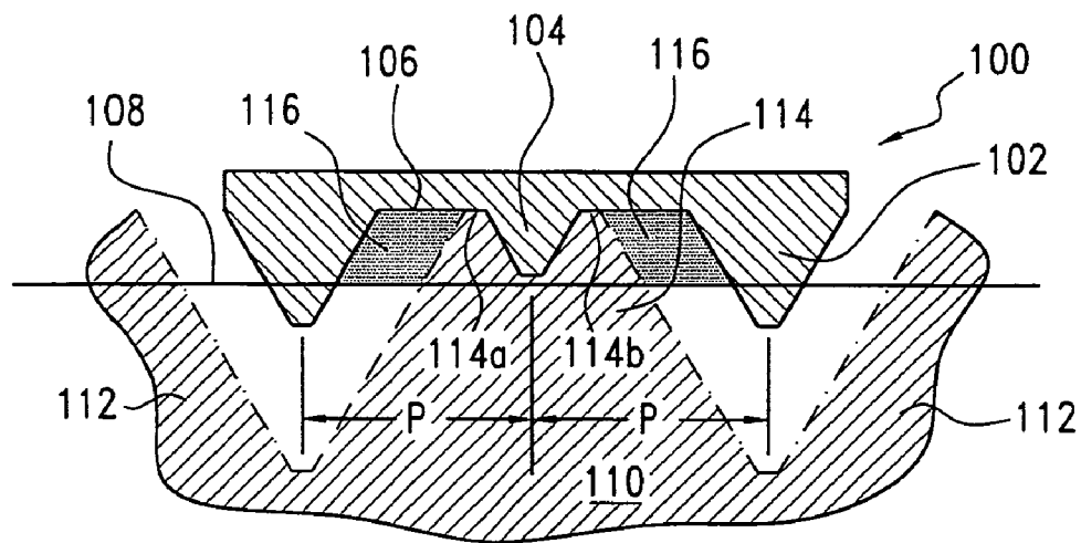
FIG. 4 (PRIOR ART)
