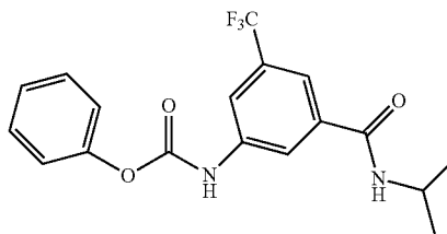
Phenyl 3-(isopropylcarbamoyl)-5-(trifluoromethyl)phenylcarbamate
