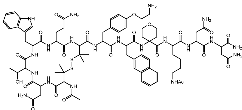
Example 2: Ac-[Pen]-NTWQ-[Pen]-[Phe[4-(2-aminoethoxy)]]-[2-Nal]-[4-amino-4-carboxy-tetrahydropyran]-[Lys(Ac)]-NN-NH 2
