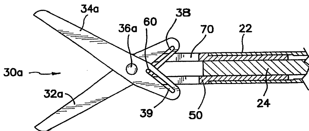
FIG. 3 PRIOR ART
