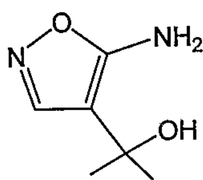
Oxazole (-0.76)
