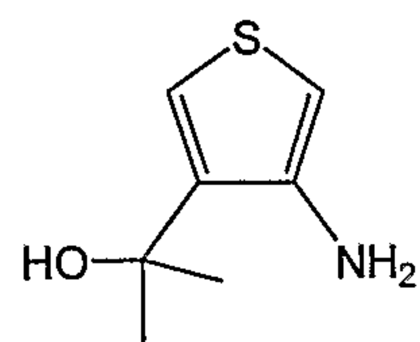
Thiophene (4.11)
