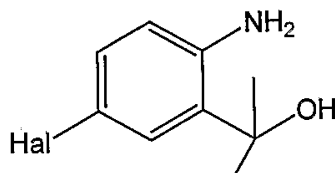
4-Bromo-benzyl alcohol (3.82)
