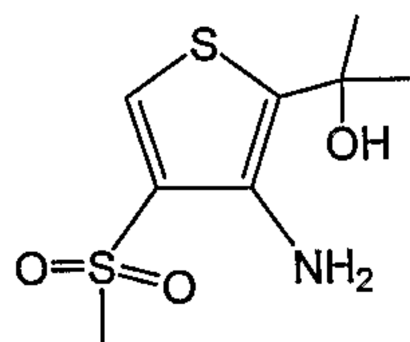
4-Methanesulfonyl-thiophene (2.26)
