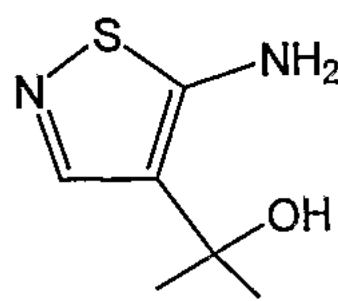
Thiazole (0.28)
