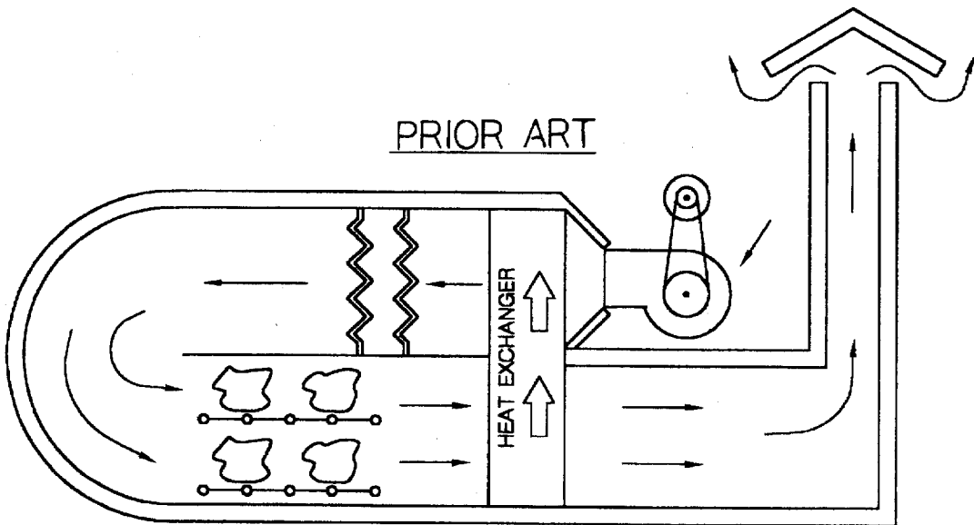
DRYER WITH HEAT RECOVERY FIGURE 1C
