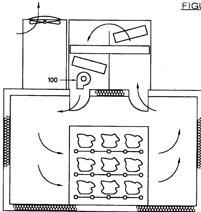
PACKAGE CEILING/ROOF MOUNTED FIGURE 7
