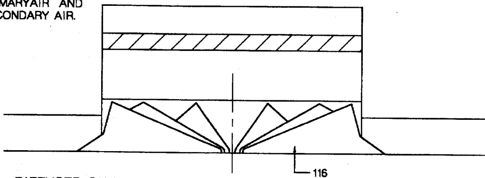
DIFFUSER SIDE VIEW
