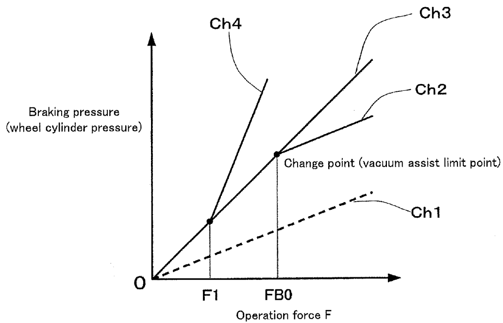
FIG. 21 Prior Art
